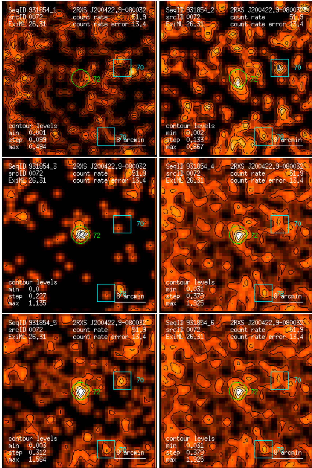
Figure 72: RASS 931854: detection 0072: band rate images, Gaussian filter: (1) PSPC channels 11 – 41, (2) 52 – 90, (3) 91 – 201, (4) 11 – 235, (5) 52 – 201, (6) 11 – 201. Broad band rates in counts/ks. Band rate contour levels in counts/ks/arcmin 2 .
