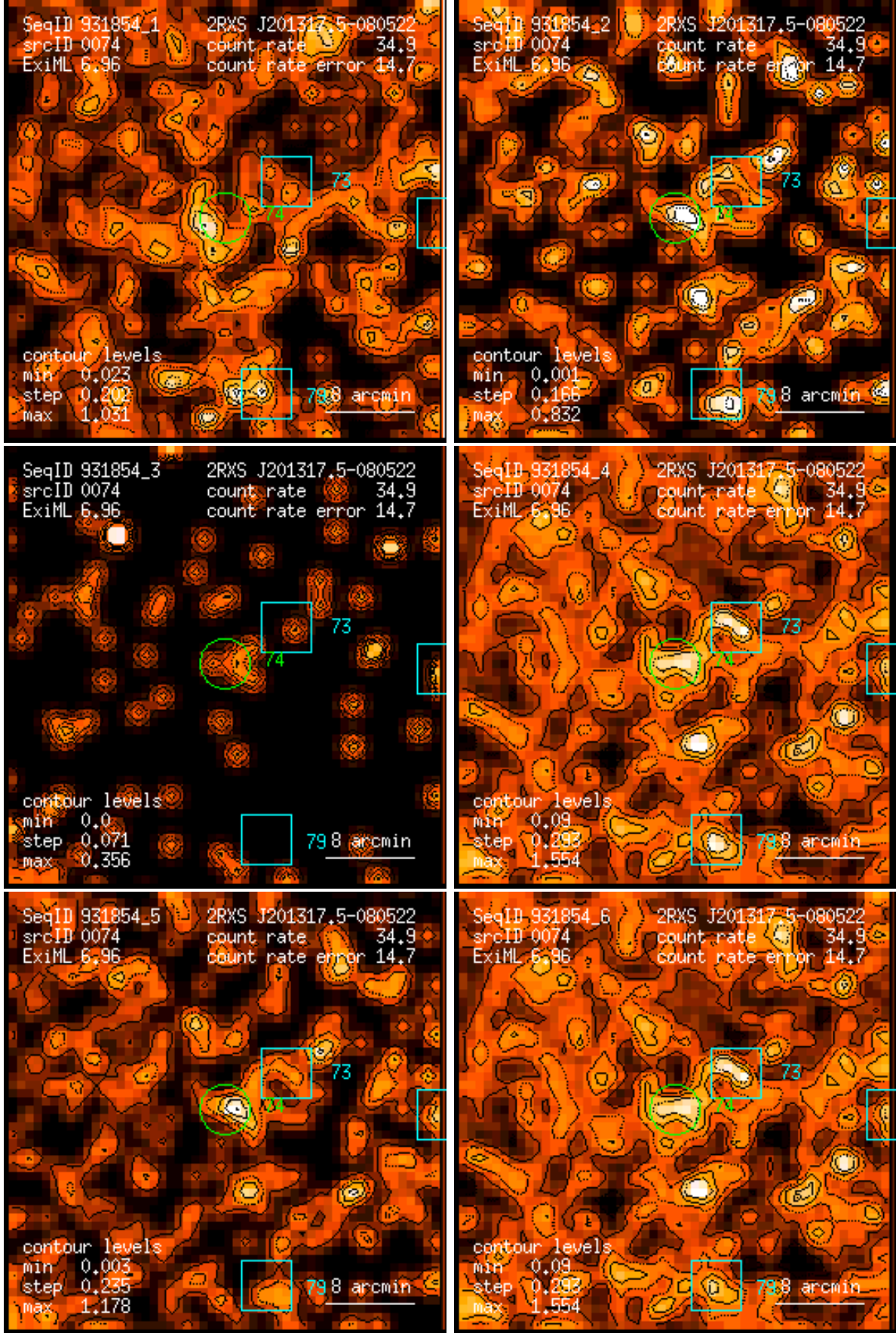
Figure 74: RASS 931854: detection 0074: band rate images, Gaussian filter: (1) PSPC channels 11 – 41, (2) 52 – 90, (3) 91 – 201, (4) 11 – 235, (5) 52 – 201, (6) 11 – 201. Broad band rates in counts/ks. Band rate contour levels in counts/ks/arcmin 2 .
