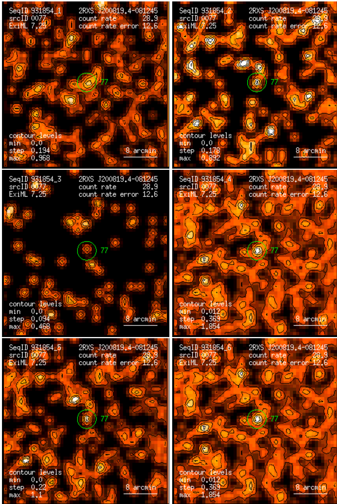
Figure 77: RASS 931854: detection 0077: band rate images, Gaussian filter: (1) PSPC channels 11 – 41, (2) 52 – 90, (3) 91 – 201, (4) 11 – 235, (5) 52 – 201, (6) 11 – 201. Broad band rates in counts/ks. Band rate contour levels in counts/ks/arcmin 2 .
