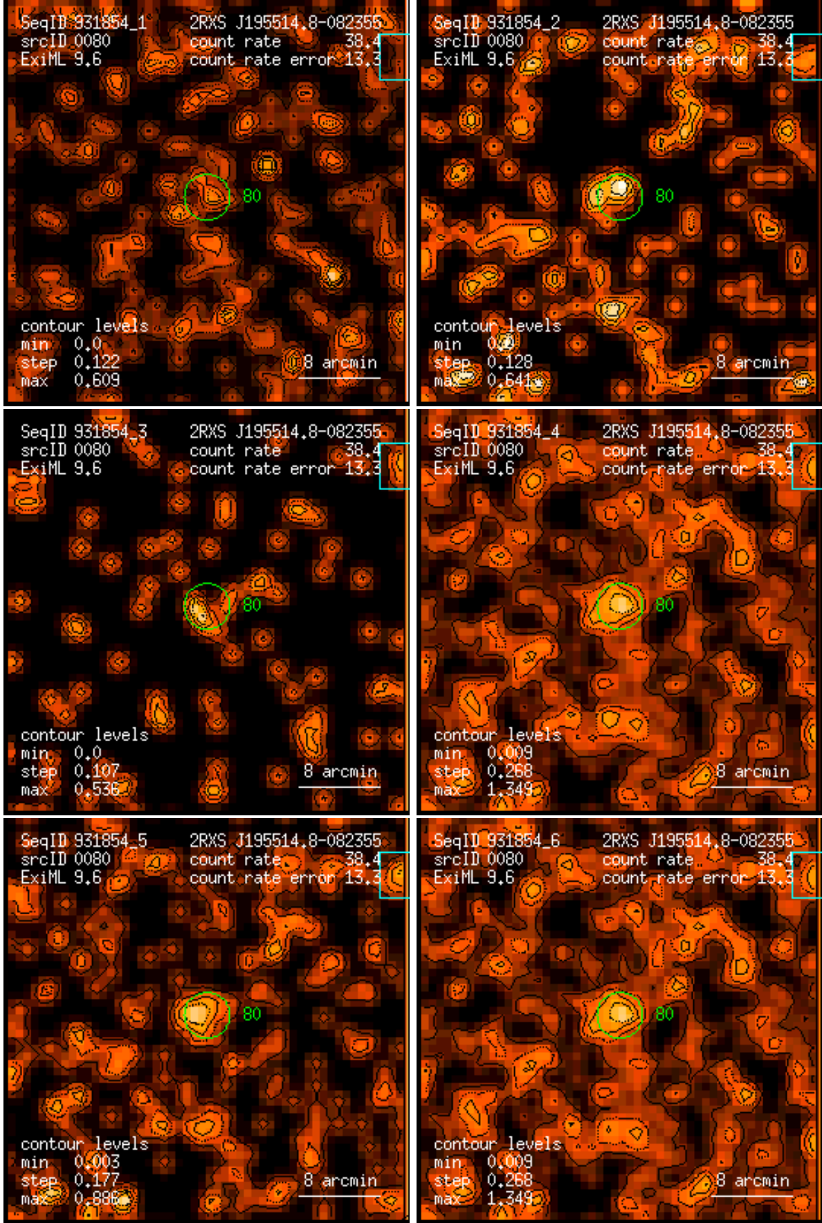
Figure 80: RASS 931854: detection 0080: band rate images, Gaussian filter: (1) PSPC channels 11 – 41, (2) 52 – 90, (3) 91 – 201, (4) 11 – 235, (5) 52 – 201, (6) 11 – 201. Broad band rates in counts/ks. Band rate contour levels in counts/ks/arcmin 2 .
