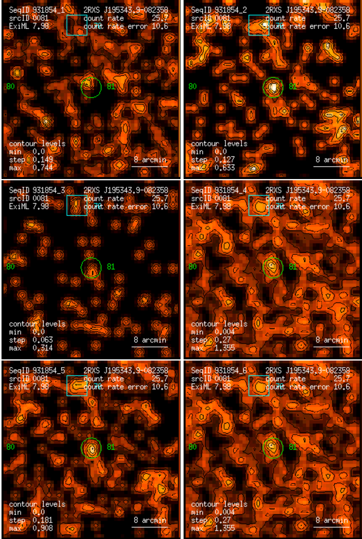
Figure 81: RASS 931854: detection 0081: band rate images, Gaussian filter: (1) PSPC channels 11 – 41, (2) 52 – 90, (3) 91 – 201, (4) 11 – 235, (5) 52 – 201, (6) 11 – 201. Broad band rates in counts/ks. Band rate contour levels in counts/ks/arcmin 2 .
