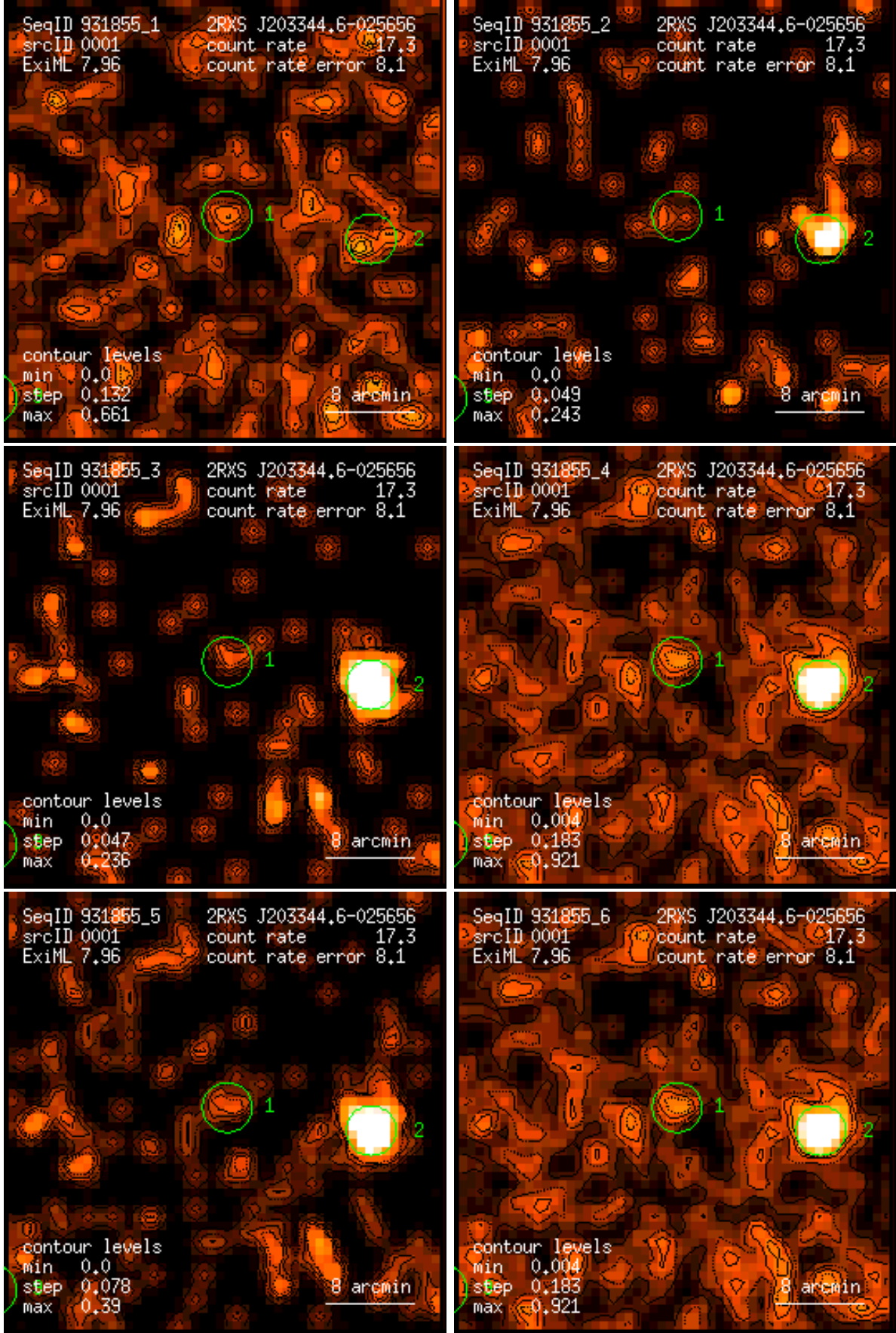
Figure 1: RASS 931855: detection 0001: band rate images, Gaussian filter: (1) PSPC channels 11 – 41, (2) 52 – 90, (3) 91 – 201, (4) 11 – 235, (5) 52 – 201, (6) 11 – 201. Broad band rates in counts/ks. Band rate contour levels in counts/ks/arcmin 2 .
