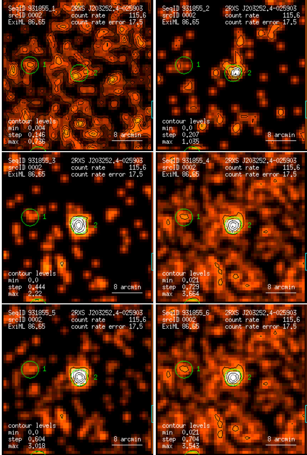
Figure 2: RASS 931855: detection 0002: band rate images, Gaussian filter: (1) PSPC channels 11 – 41, (2) 52 – 90, (3) 91 – 201, (4) 11 – 235, (5) 52 – 201, (6) 11 – 201. Broad band rates in counts/ks. Band rate contour levels in counts/ks/arcmin 2 .
