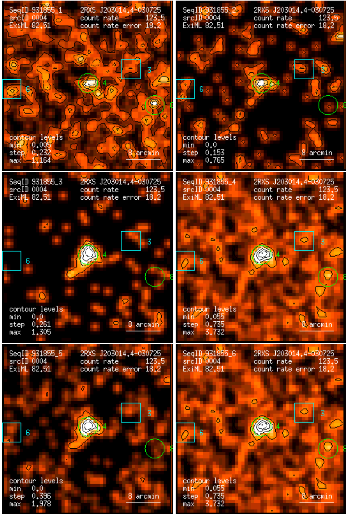
Figure 4: RASS 931855: detection 0004: band rate images, Gaussian filter: (1) PSPC channels 11 – 41, (2) 52 – 90, (3) 91 – 201, (4) 11 – 235, (5) 52 – 201, (6) 11 – 201. Broad band rates in counts/ks. Band rate contour levels in counts/ks/arcmin 2 .
