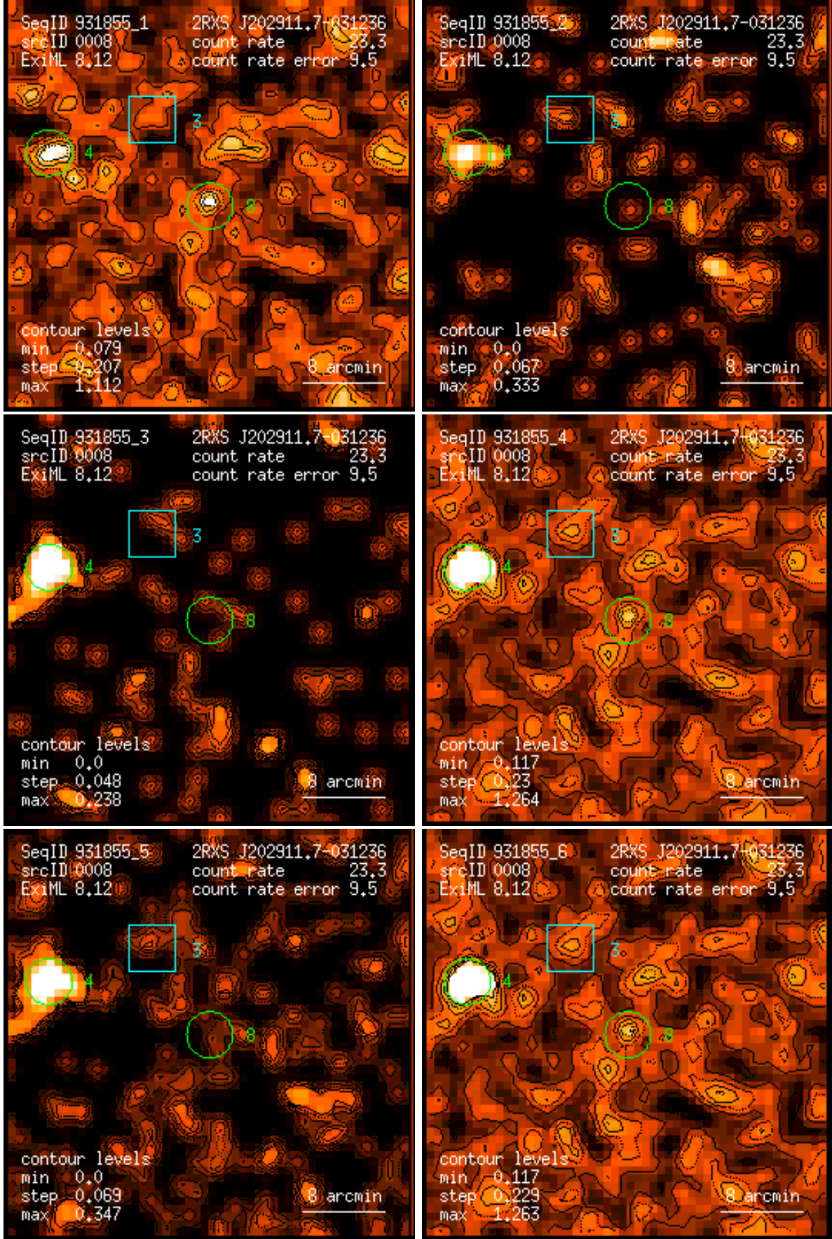
Figure 8: RASS 931855: detection 0008: band rate images, Gaussian filter: (1) PSPC channels 11 – 41, (2) 52 – 90, (3) 91 – 201, (4) 11 – 235, (5) 52 – 201, (6) 11 – 201. Broad band rates in counts/ks. Band rate contour levels in counts/ks/arcmin 2 .
