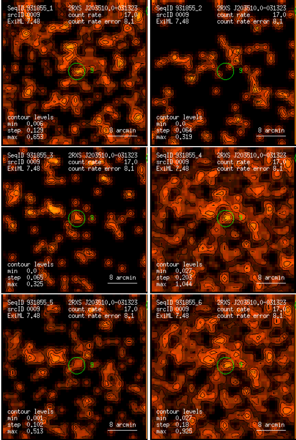
Figure 9: RASS 931855: detection 0009: band rate images, Gaussian filter: (1) PSPC channels 11 – 41, (2) 52 – 90, (3) 91 – 201, (4) 11 – 235, (5) 52 – 201, (6) 11 – 201. Broad band rates in counts/ks. Band rate contour levels in counts/ks/arcmin 2 .
