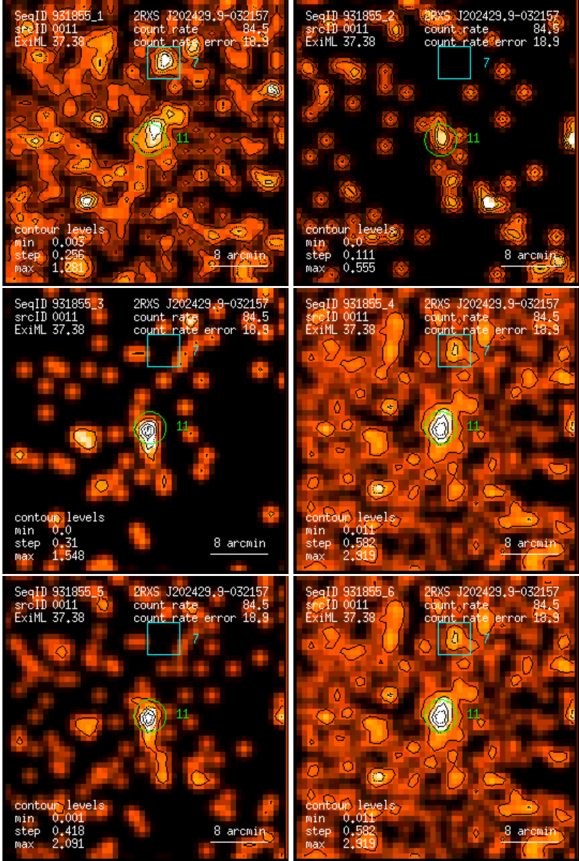
Figure 11: RASS 931855: detection 0011: band rate images, Gaussian filter: (1) PSPC channels 11 – 41, (2) 52 – 90, (3) 91 – 201, (4) 11 – 235, (5) 52 – 201, (6) 11 – 201. Broad band rates in counts/ks. Band rate contour levels in counts/ks/arcmin 2 .
