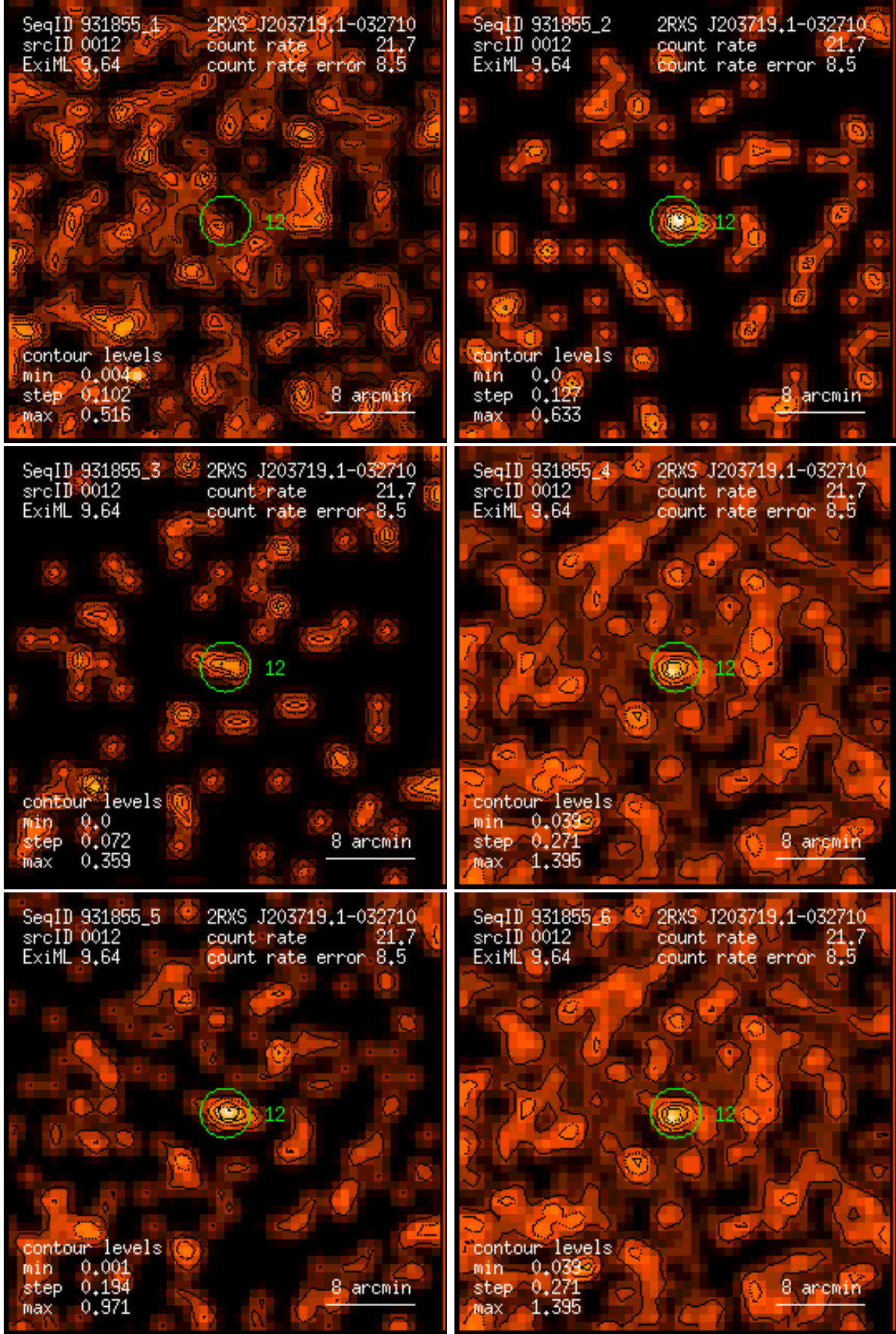
Figure 12: RASS 931855: detection 0012: band rate images, Gaussian filter: (1) PSPC channels 11 – 41, (2) 52 – 90, (3) 91 – 201, (4) 11 – 235, (5) 52 – 201, (6) 11 – 201. Broad band rates in counts/ks. Band rate contour levels in counts/ks/arcmin 2 .
