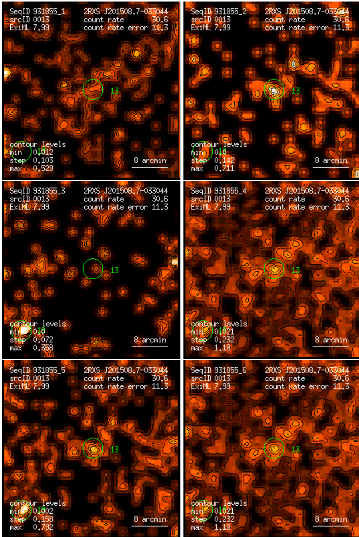
Figure 13: RASS 931855: detection 0013: band rate images, Gaussian filter: (1) PSPC channels 11 – 41, (2) 52 – 90, (3) 91 – 201, (4) 11 – 235, (5) 52 – 201, (6) 11 – 201. Broad band rates in counts/ks. Band rate contour levels in counts/ks/arcmin 2 .
