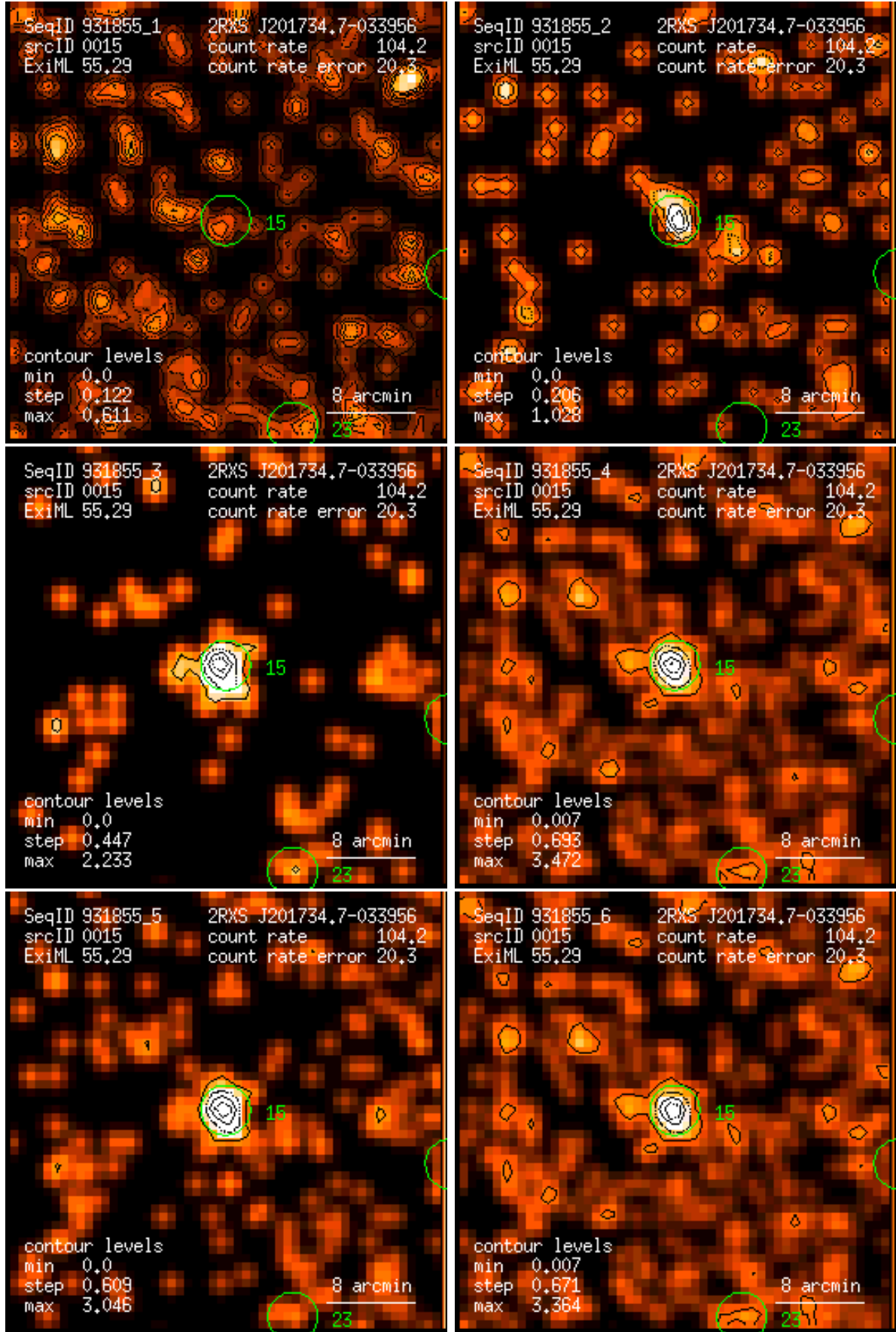
Figure 15: RASS 931855: detection 0015: band rate images, Gaussian filter: (1) PSPC channels 11 – 41, (2) 52 – 90, (3) 91 – 201, (4) 11 – 235, (5) 52 – 201, (6) 11 – 201. Broad band rates in counts/ks. Band rate contour levels in counts/ks/arcmin 2 .
