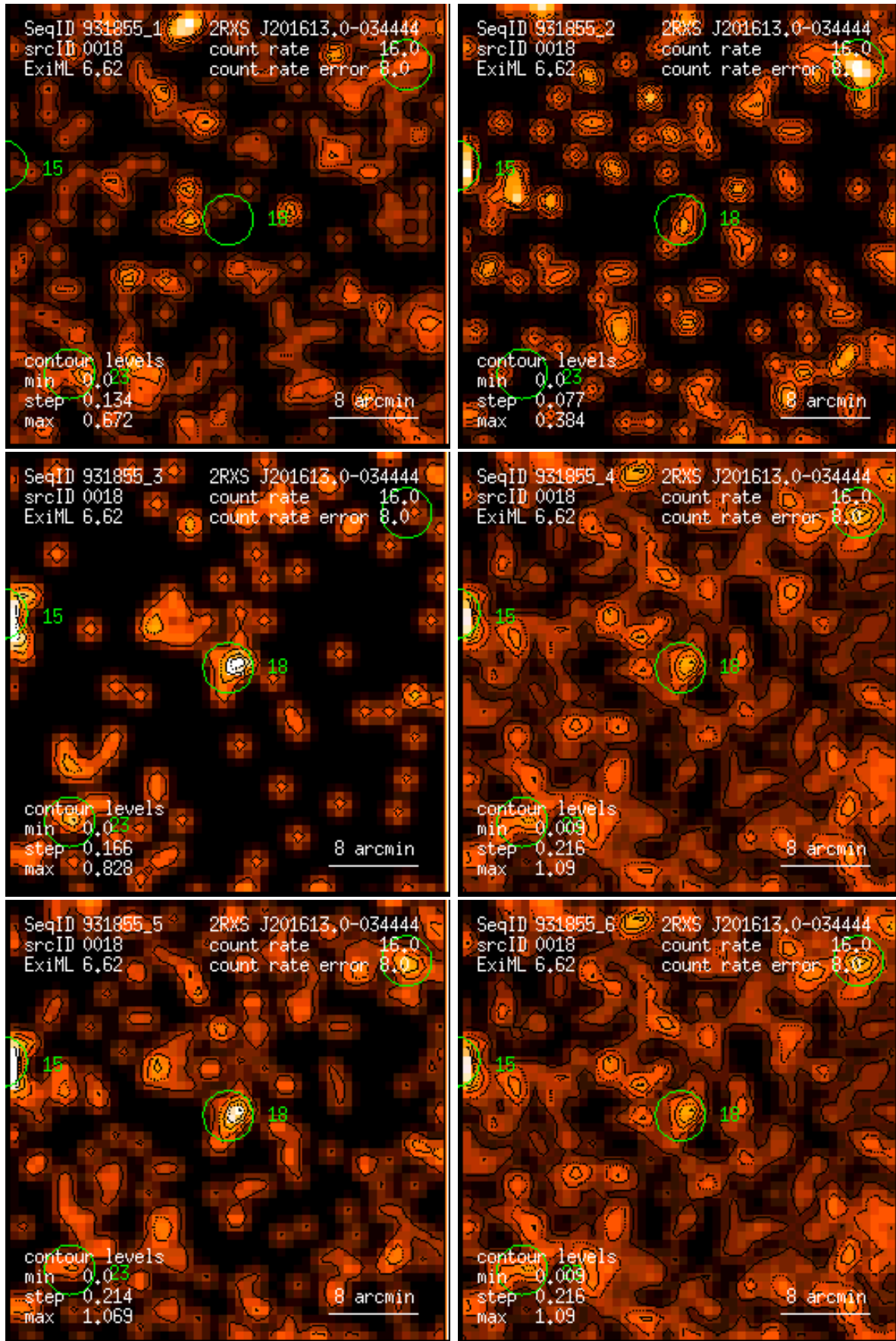
Figure 18: RASS 931855: detection 0018: band rate images, Gaussian filter: (1) PSPC channels 11 – 41, (2) 52 – 90, (3) 91 – 201, (4) 11 – 235, (5) 52 – 201, (6) 11 – 201. Broad band rates in counts/ks. Band rate contour levels in counts/ks/arcmin 2 .
