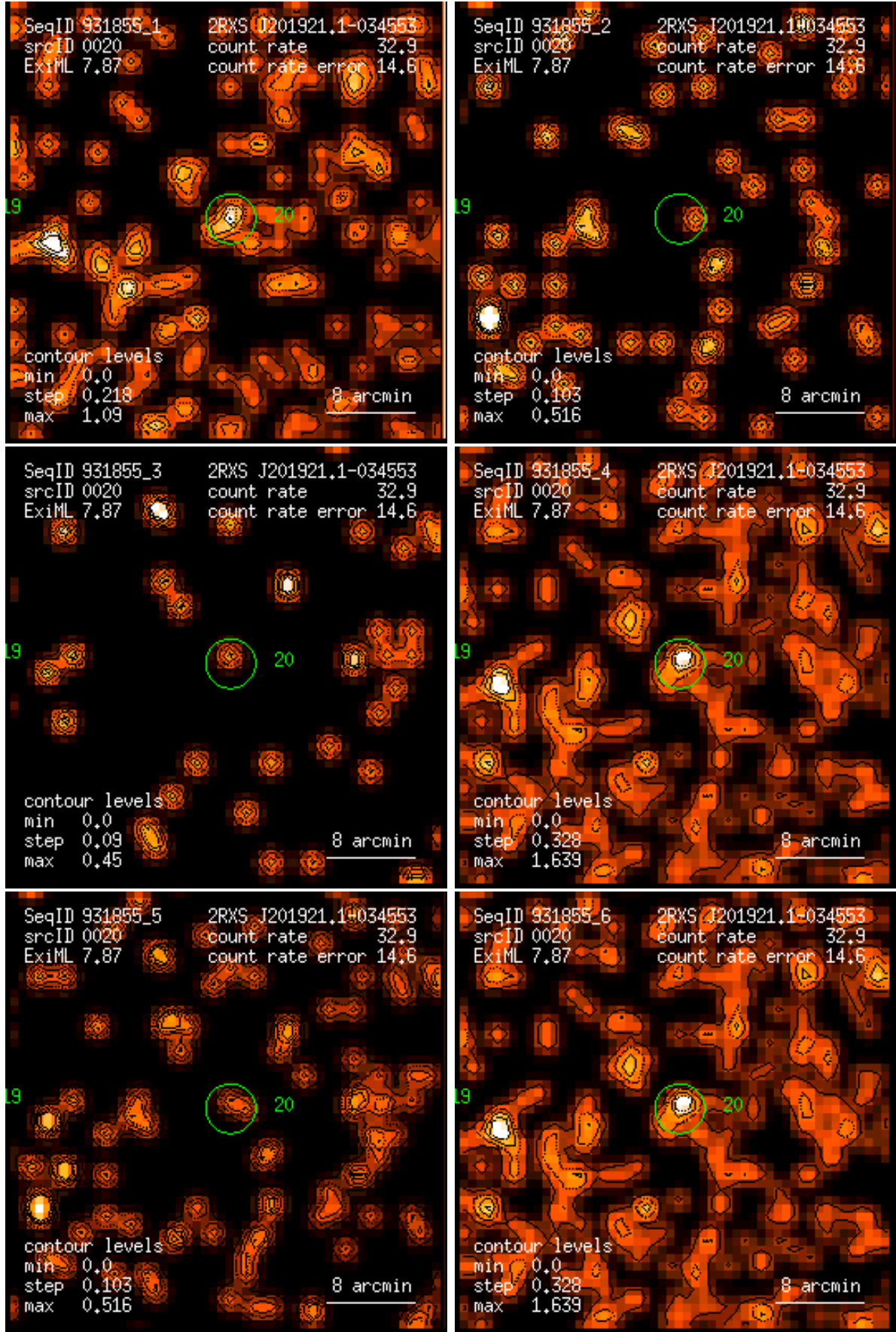
Figure 20: RASS 931855: detection 0020: band rate images, Gaussian filter: (1) PSPC channels 11 – 41, (2) 52 – 90, (3) 91 – 201, (4) 11 – 235, (5) 52 – 201, (6) 11 – 201. Broad band rates in counts/ks. Band rate contour levels in counts/ks/arcmin 2 .
