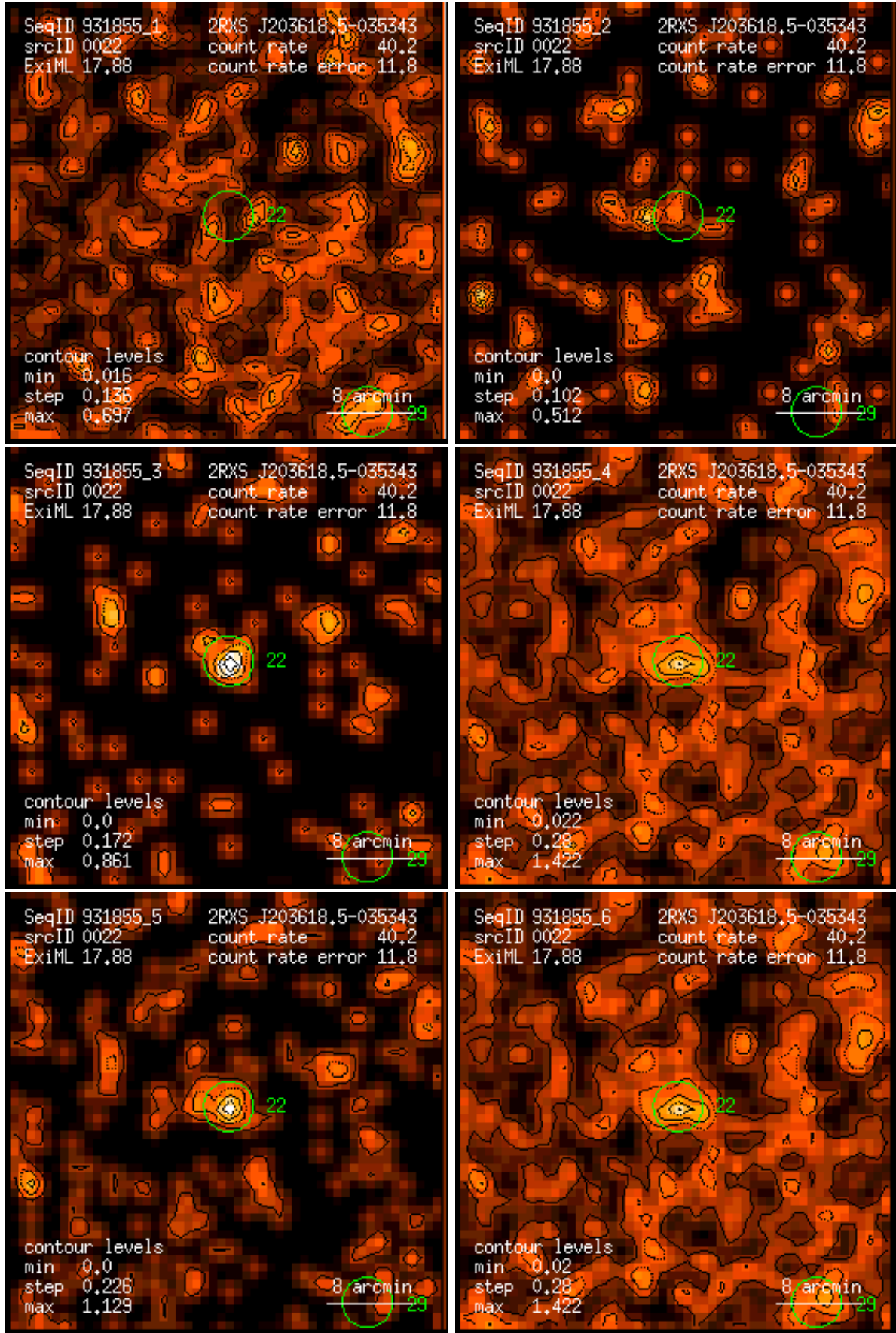
Figure 22: RASS 931855: detection 0022: band rate images, Gaussian filter: (1) PSPC channels 11 – 41, (2) 52 – 90, (3) 91 – 201, (4) 11 – 235, (5) 52 – 201, (6) 11 – 201. Broad band rates in counts/ks. Band rate contour levels in counts/ks/arcmin 2 .
