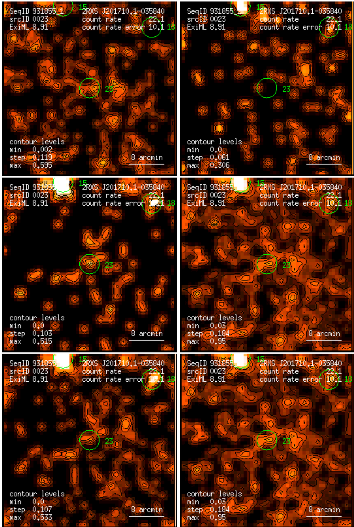
Figure 23: RASS 931855: detection 0023: band rate images, Gaussian filter: (1) PSPC channels 11 – 41, (2) 52 – 90, (3) 91 – 201, (4) 11 – 235, (5) 52 – 201, (6) 11 – 201. Broad band rates in counts/ks. Band rate contour levels in counts/ks/arcmin 2 .
