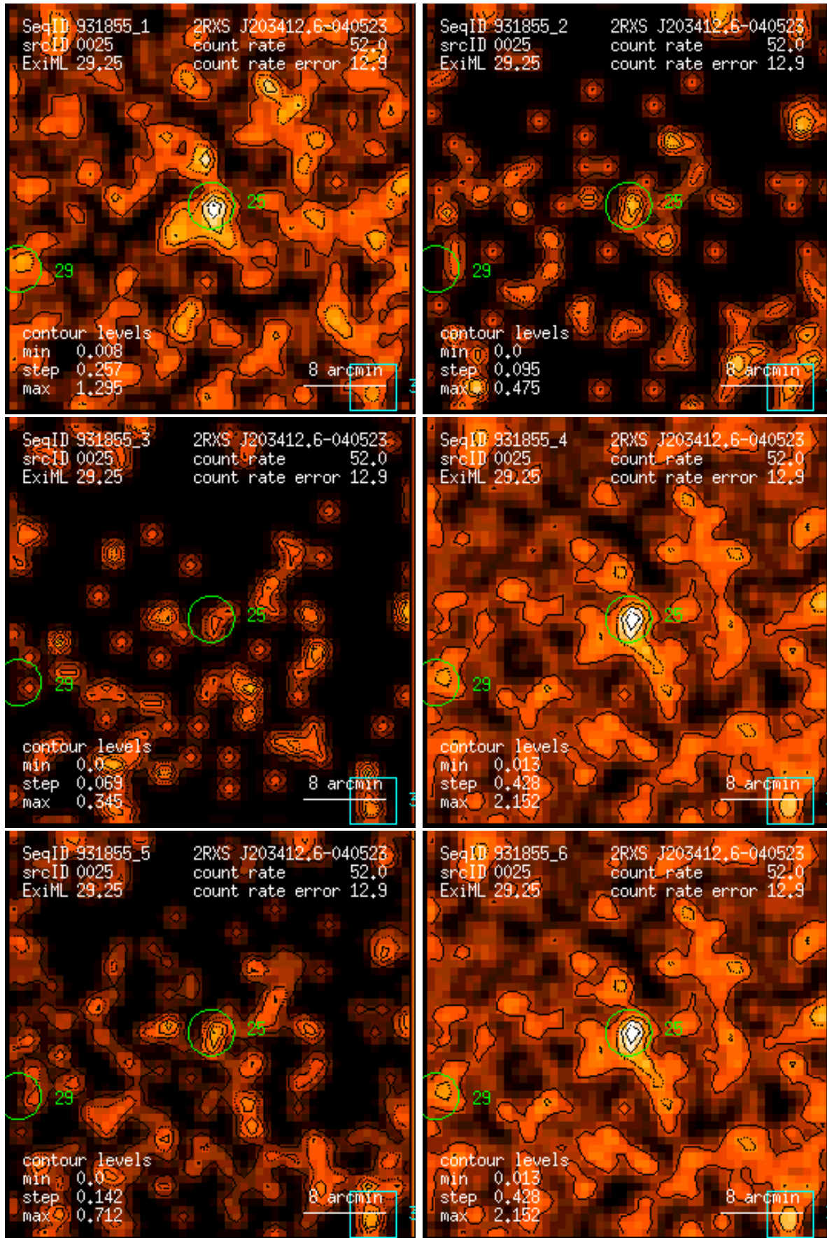
Figure 25: RASS 931855: detection 0025: band rate images, Gaussian filter: (1) PSPC channels 11 – 41, (2) 52 – 90, (3) 91 – 201, (4) 11 – 235, (5) 52 – 201, (6) 11 – 201. Broad band rates in counts/ks. Band rate contour levels in counts/ks/arcmin 2 .
