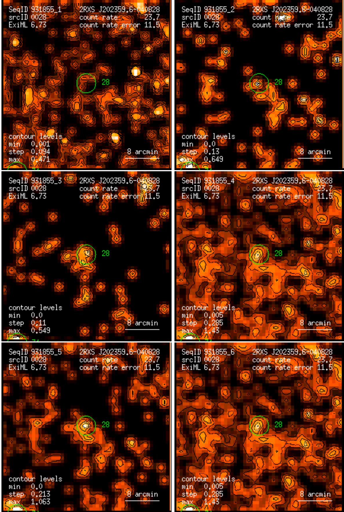
Figure 28: RASS 931855: detection 0028: band rate images, Gaussian filter: (1) PSPC channels 11 – 41, (2) 52 – 90, (3) 91 – 201, (4) 11 – 235, (5) 52 – 201, (6) 11 – 201. Broad band rates in counts/ks. Band rate contour levels in counts/ks/arcmin 2 .
