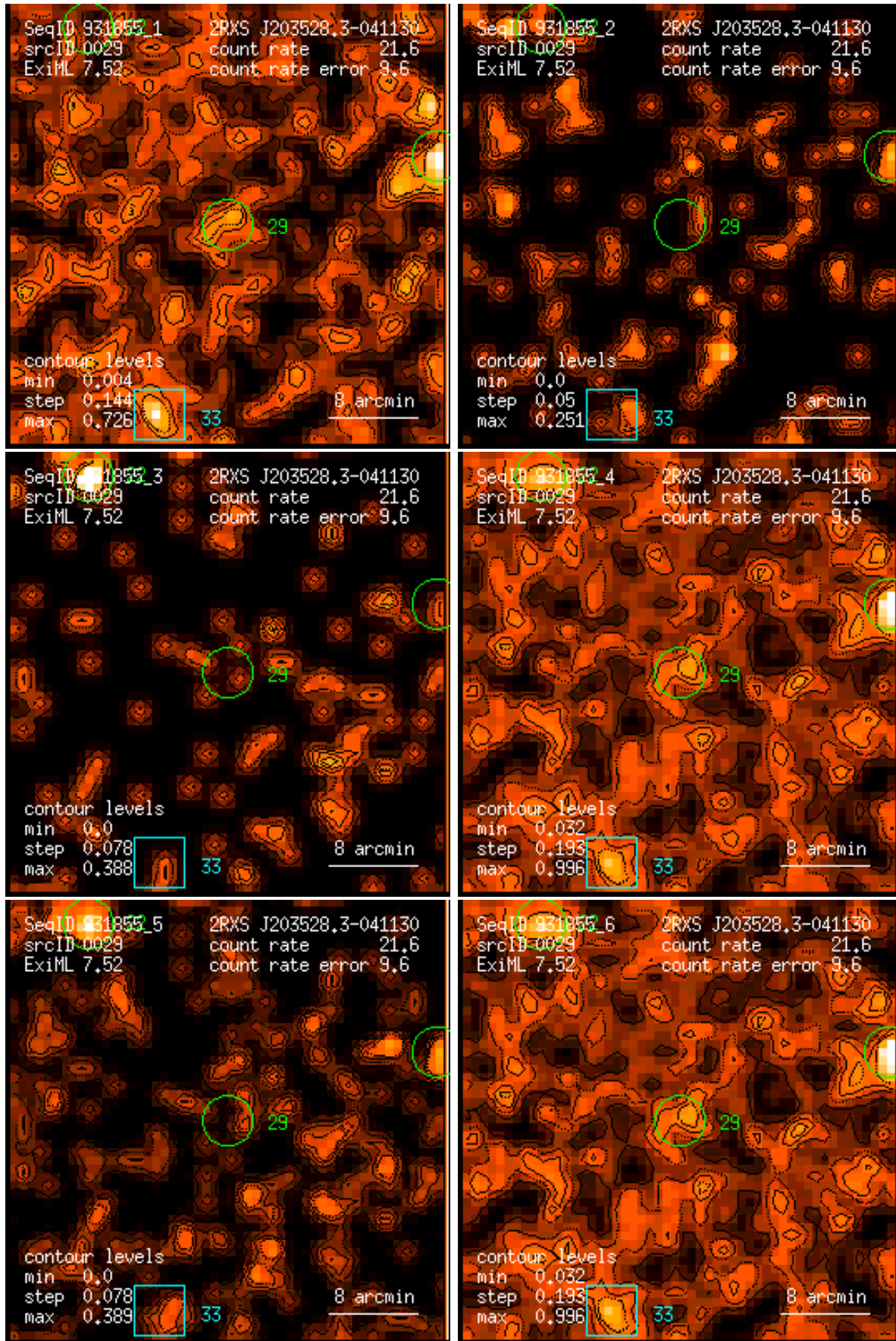
Figure 29: RASS 931855: detection 0029: band rate images, Gaussian filter: (1) PSPC channels 11 – 41, (2) 52 – 90, (3) 91 – 201, (4) 11 – 235, (5) 52 – 201, (6) 11 – 201. Broad band rates in counts/ks. Band rate contour levels in counts/ks/arcmin 2 .
