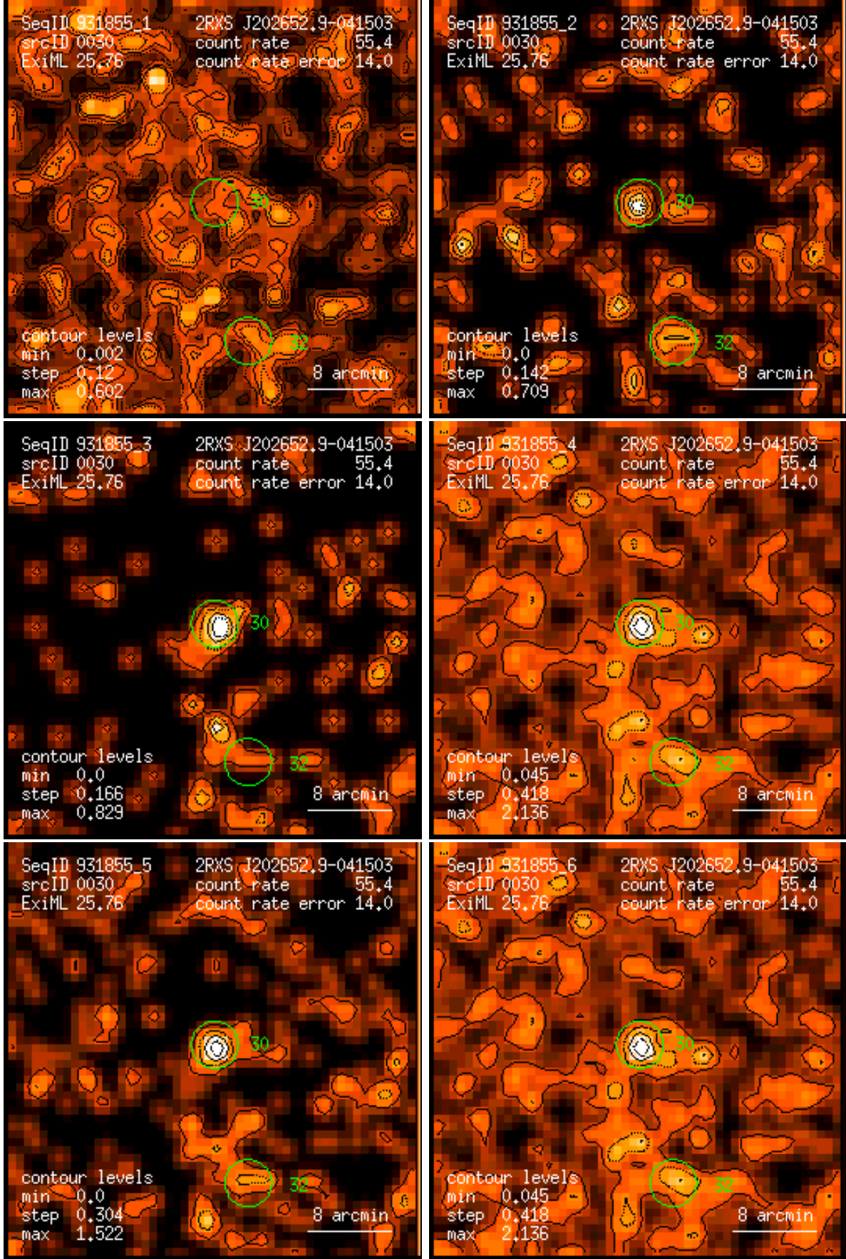
Figure 30: RASS 931855: detection 0030: band rate images, Gaussian filter: (1) PSPC channels 11 – 41, (2) 52 – 90, (3) 91 – 201, (4) 11 – 235, (5) 52 – 201, (6) 11 – 201. Broad band rates in counts/ks. Band rate contour levels in counts/ks/arcmin 2 .
