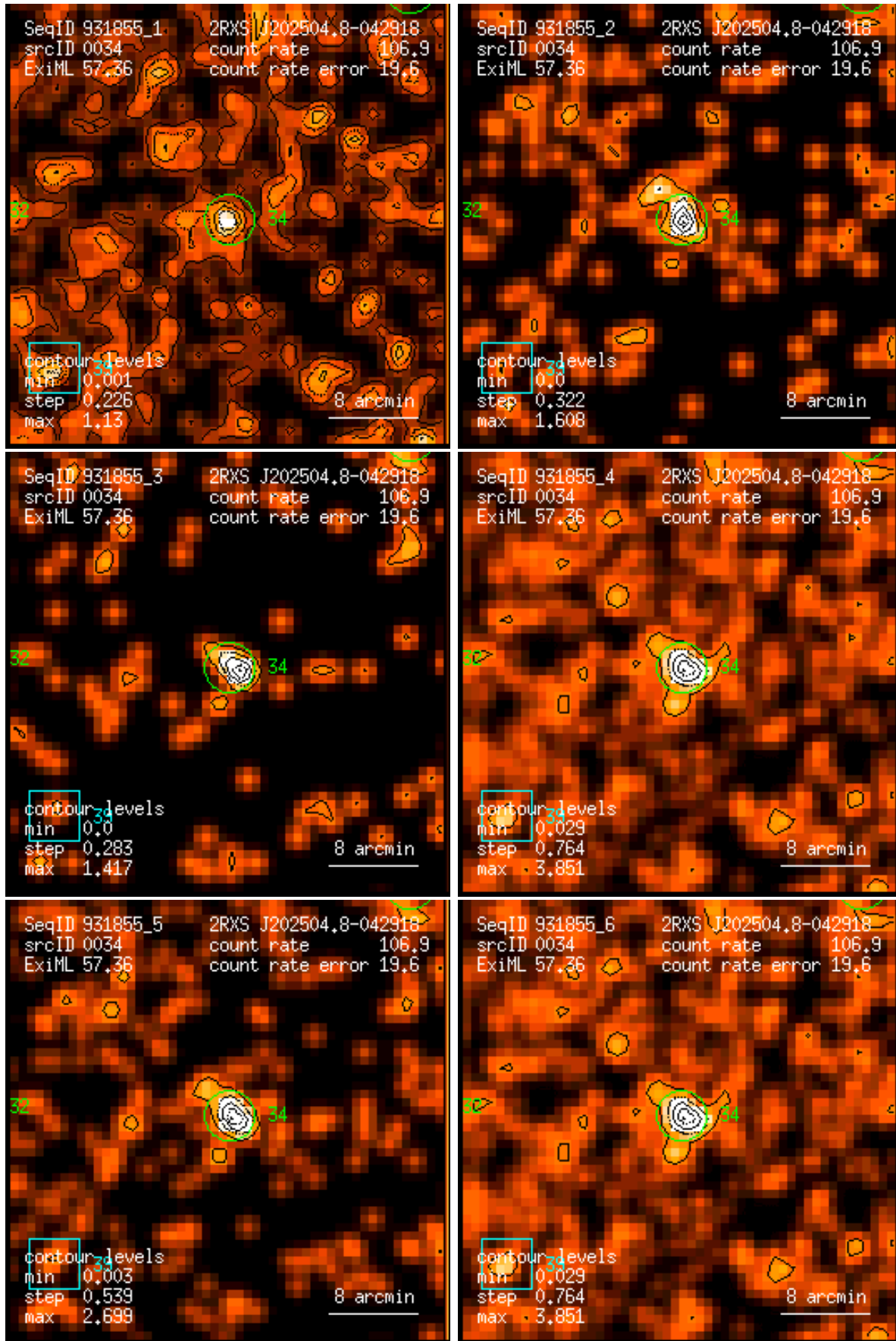
Figure 34: RASS 931855: detection 0034: band rate images, Gaussian filter: (1) PSPC channels 11 – 41, (2) 52 – 90, (3) 91 – 201, (4) 11 – 235, (5) 52 – 201, (6) 11 – 201. Broad band rates in counts/ks. Band rate contour levels in counts/ks/arcmin 2 .
