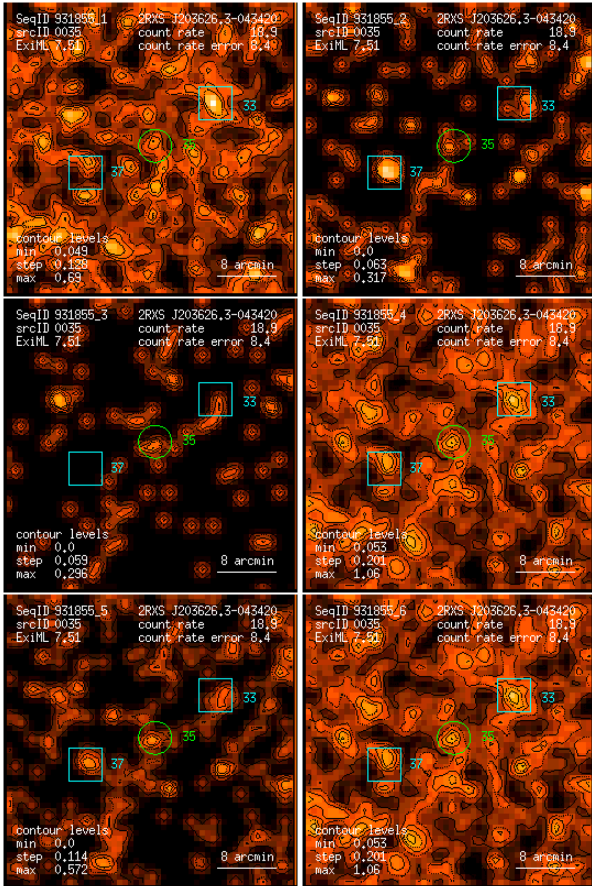
Figure 35: RASS 931855: detection 0035: band rate images, Gaussian filter: (1) PSPC channels 11 – 41, (2) 52 – 90, (3) 91 – 201, (4) 11 – 235, (5) 52 – 201, (6) 11 – 201. Broad band rates in counts/ks. Band rate contour levels in counts/ks/arcmin 2 .
