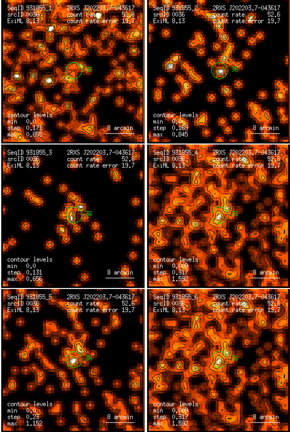
Figure 36: RASS 931855: detection 0036: band rate images, Gaussian filter: (1) PSPC channels 11 – 41, (2) 52 – 90, (3) 91 – 201, (4) 11 – 235, (5) 52 – 201, (6) 11 – 201. Broad band rates in counts/ks. Band rate contour levels in counts/ks/arcmin 2 .
