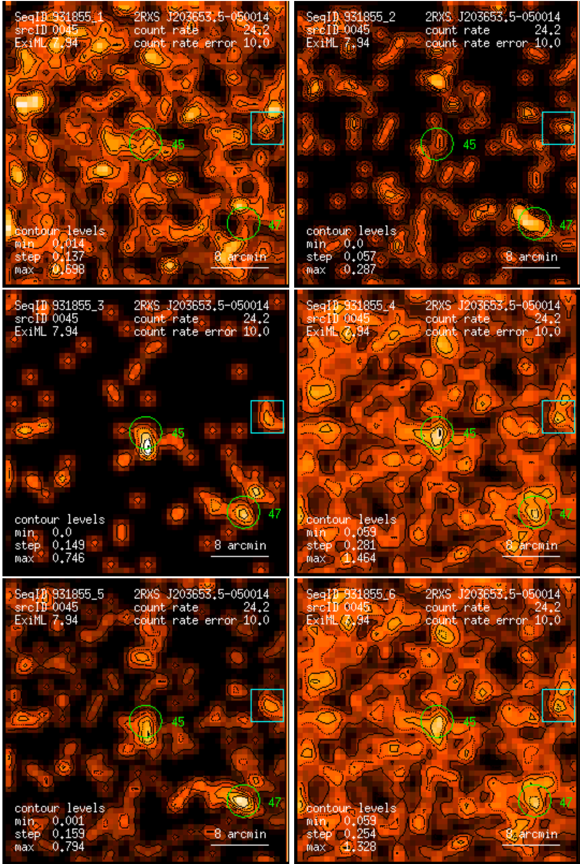
Figure 45: RASS 931855: detection 0045: band rate images, Gaussian filter: (1) PSPC channels 11 – 41, (2) 52 – 90, (3) 91 – 201, (4) 11 – 235, (5) 52 – 201, (6) 11 – 201. Broad band rates in counts/ks. Band rate contour levels in counts/ks/arcmin 2 .
