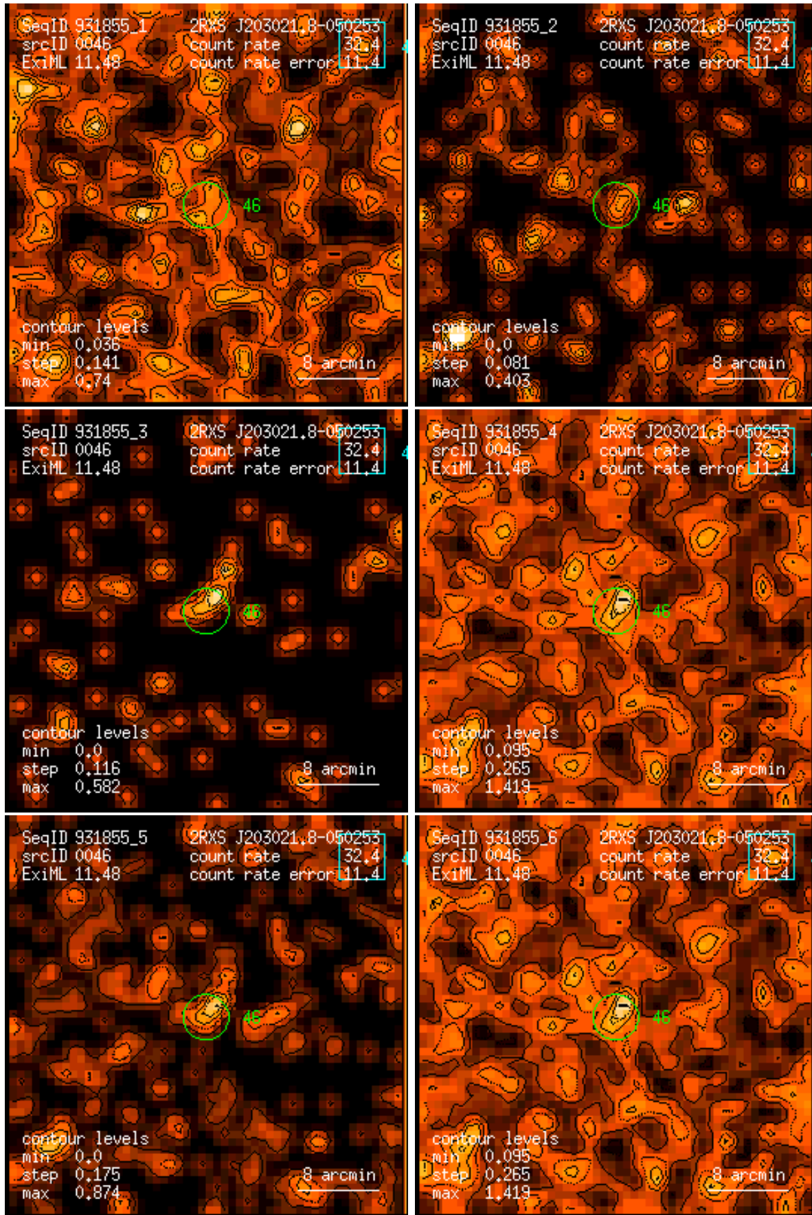
Figure 46: RASS 931855: detection 0046: band rate images, Gaussian filter: (1) PSPC channels 11 – 41, (2) 52 – 90, (3) 91 – 201, (4) 11 – 235, (5) 52 – 201, (6) 11 – 201. Broad band rates in counts/ks. Band rate contour levels in counts/ks/arcmin 2 .
