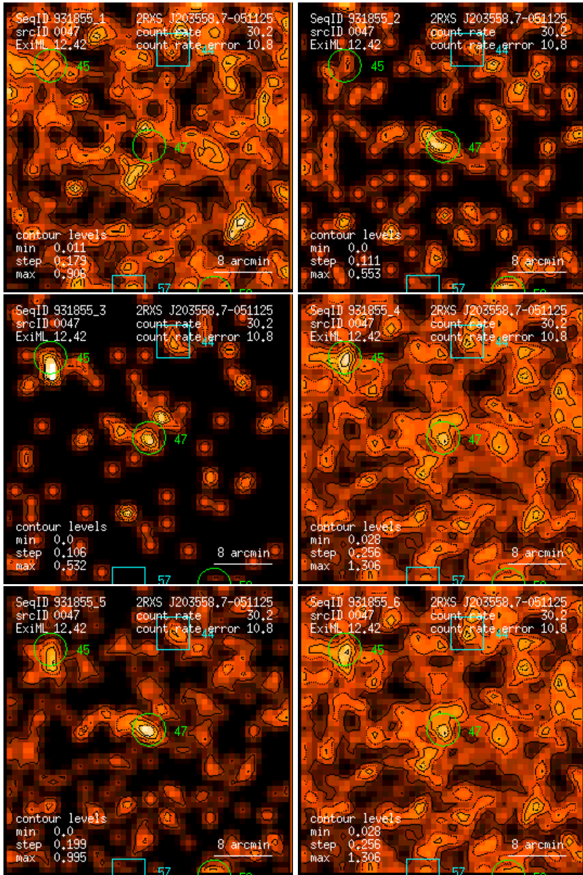
Figure 47: RASS 931855: detection 0047: band rate images, Gaussian filter: (1) PSPC channels 11 – 41, (2) 52 – 90, (3) 91 – 201, (4) 11 – 235, (5) 52 – 201, (6) 11 – 201. Broad band rates in counts/ks. Band rate contour levels in counts/ks/arcmin 2 .
