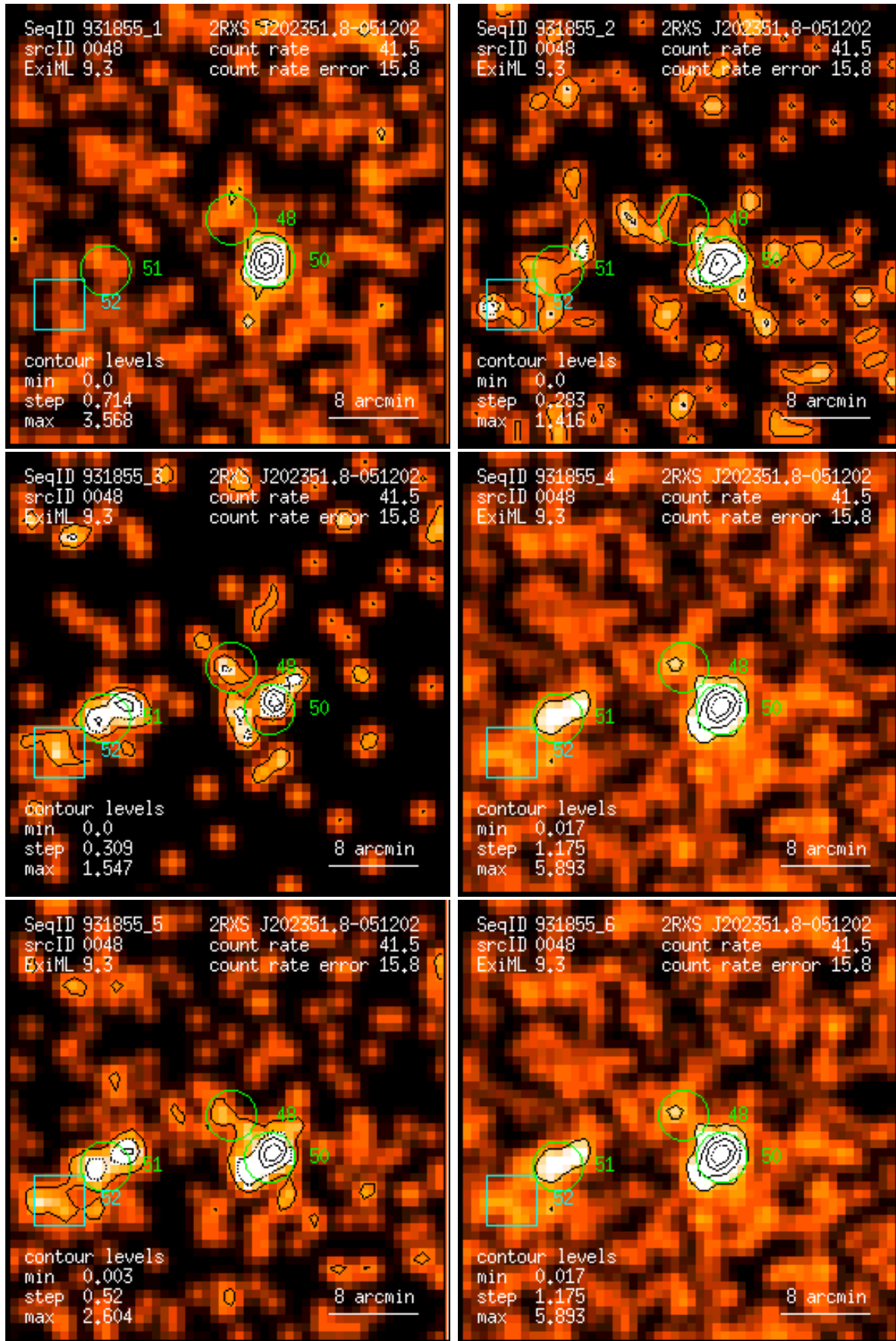
Figure 48: RASS 931855: detection 0048: band rate images, Gaussian filter: (1) PSPC channels 11 – 41, (2) 52 – 90, (3) 91 – 201, (4) 11 – 235, (5) 52 – 201, (6) 11 – 201. Broad band rates in counts/ks. Band rate contour levels in counts/ks/arcmin 2 .
