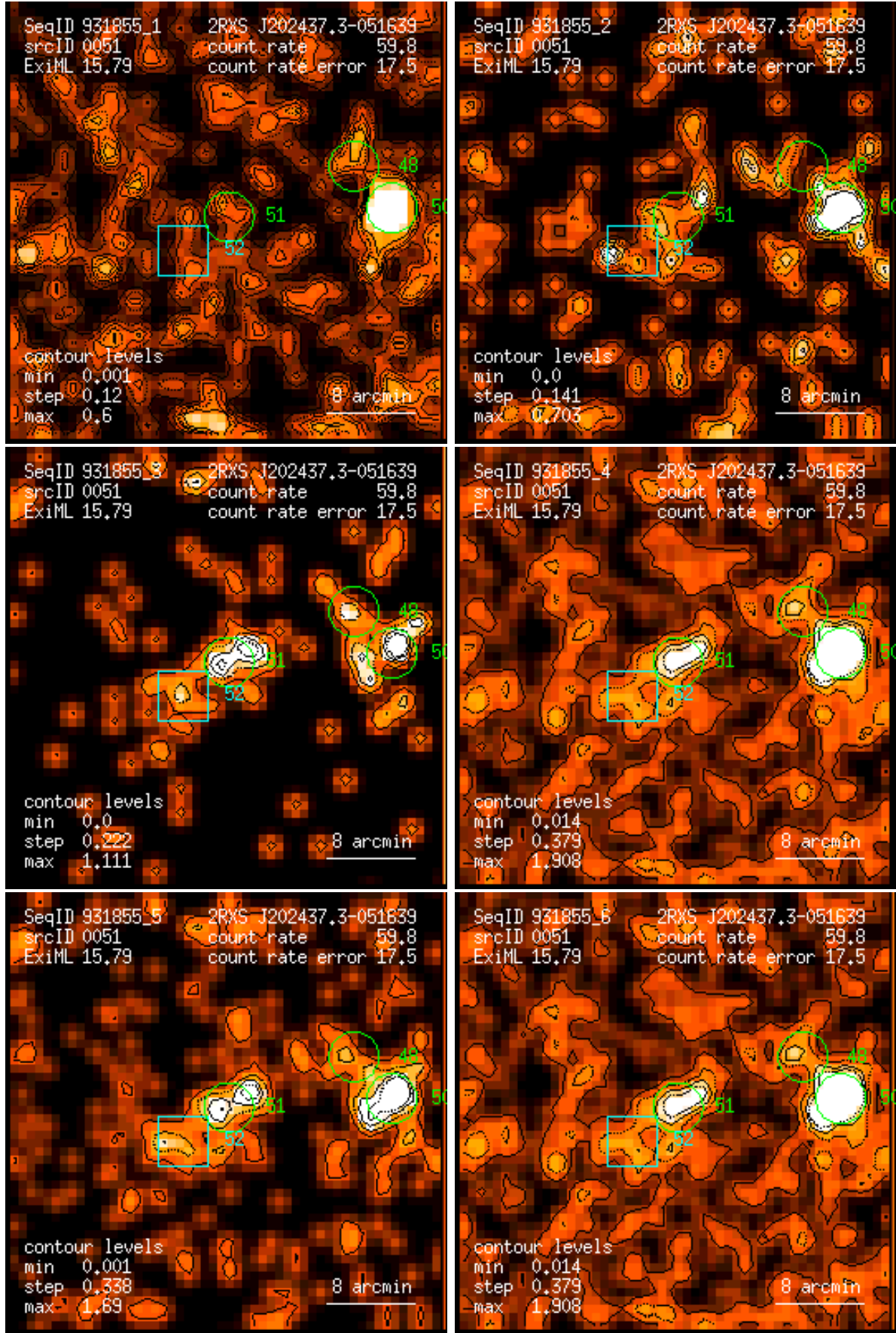
Figure 51: RASS 931855: detection 0051: band rate images, Gaussian filter: (1) PSPC channels 11 – 41, (2) 52 – 90, (3) 91 – 201, (4) 11 – 235, (5) 52 – 201, (6) 11 – 201. Broad band rates in counts/ks. Band rate contour levels in counts/ks/arcmin 2 .
