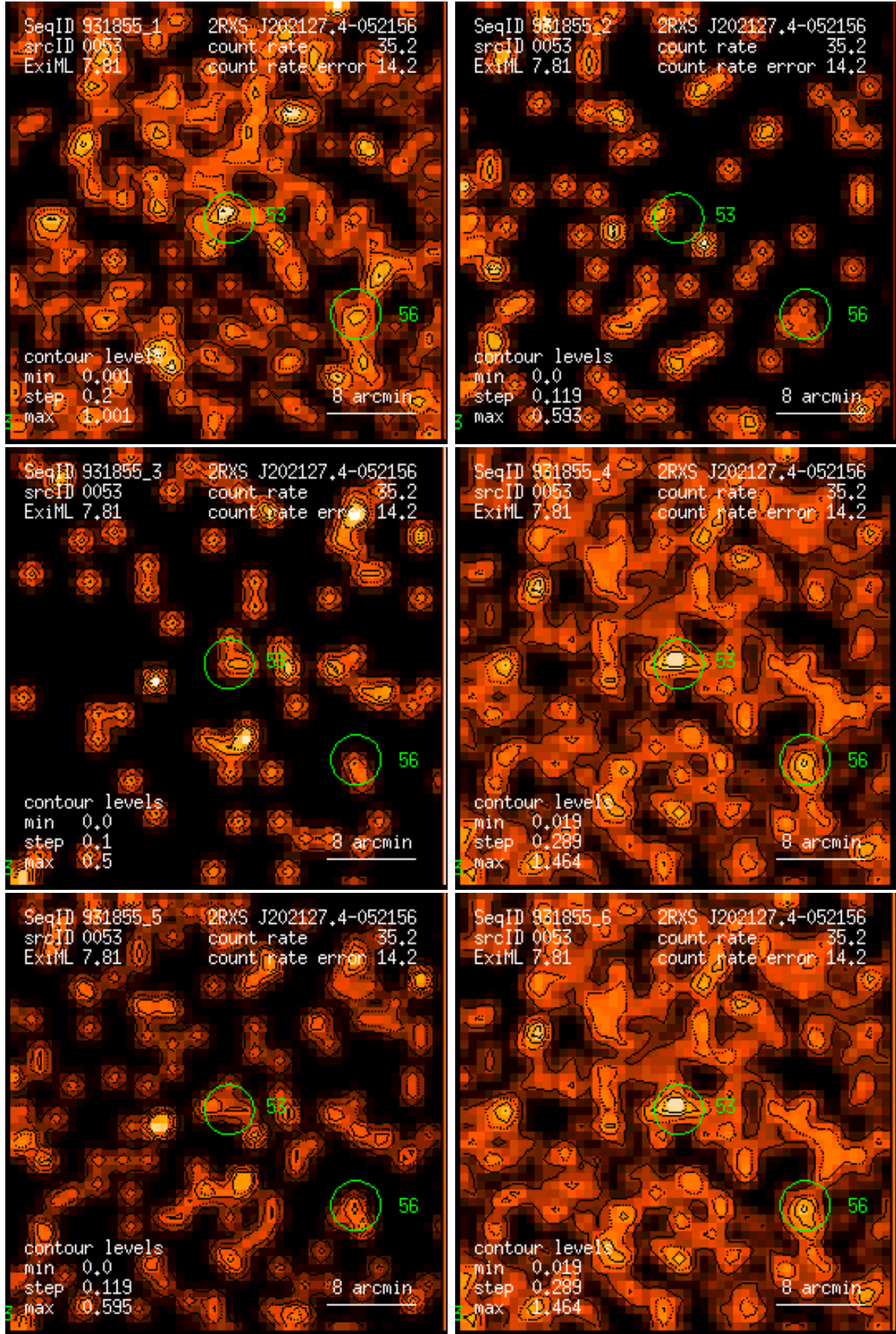
Figure 53: RASS 931855: detection 0053: band rate images, Gaussian filter: (1) PSPC channels 11 – 41, (2) 52 – 90, (3) 91 – 201, (4) 11 – 235, (5) 52 – 201, (6) 11 – 201. Broad band rates in counts/ks. Band rate contour levels in counts/ks/arcmin 2 .
