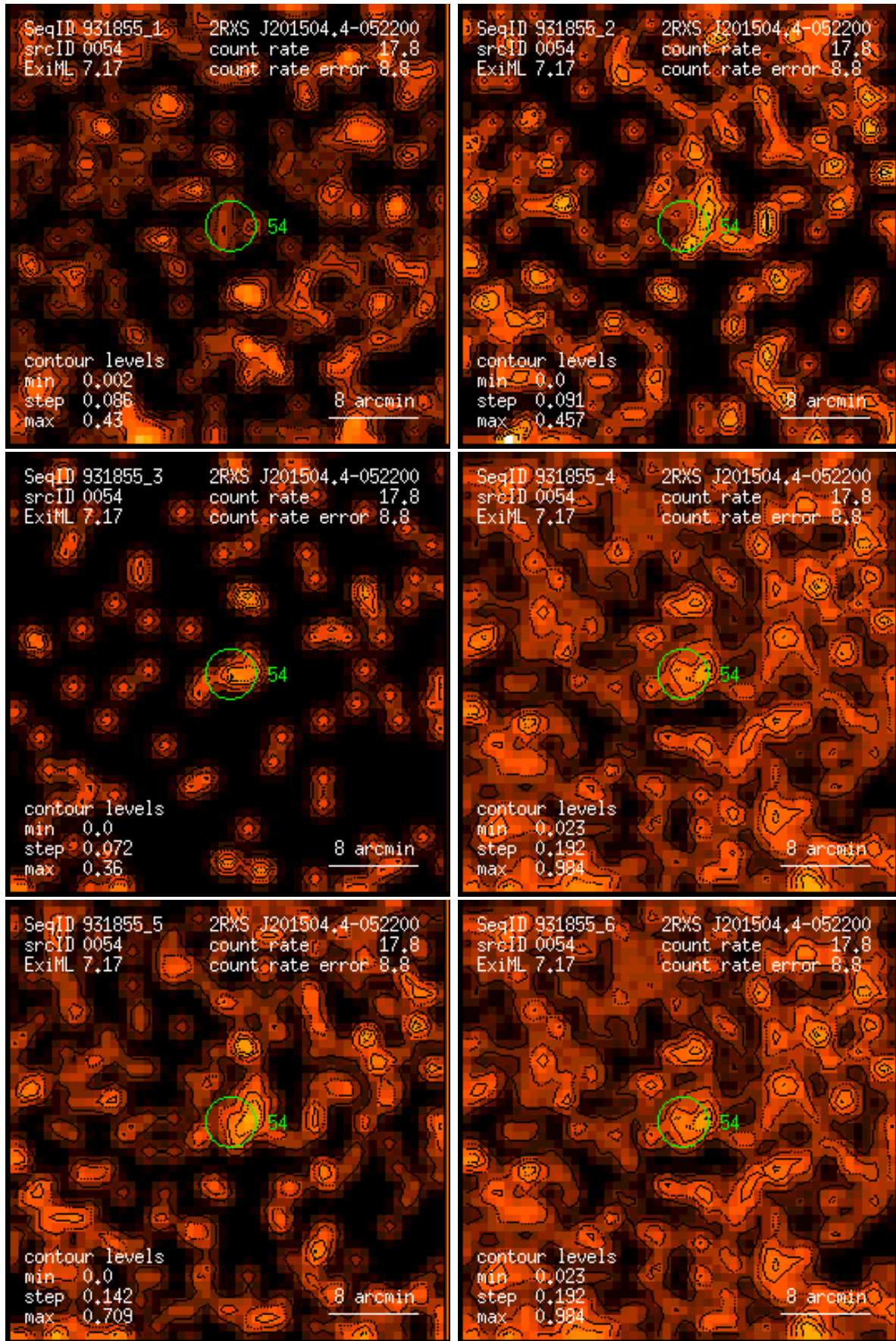
Figure 54: RASS 931855: detection 0054: band rate images, Gaussian filter: (1) PSPC channels 11 – 41, (2) 52 – 90, (3) 91 – 201, (4) 11 – 235, (5) 52 – 201, (6) 11 – 201. Broad band rates in counts/ks. Band rate contour levels in counts/ks/arcmin 2 .
