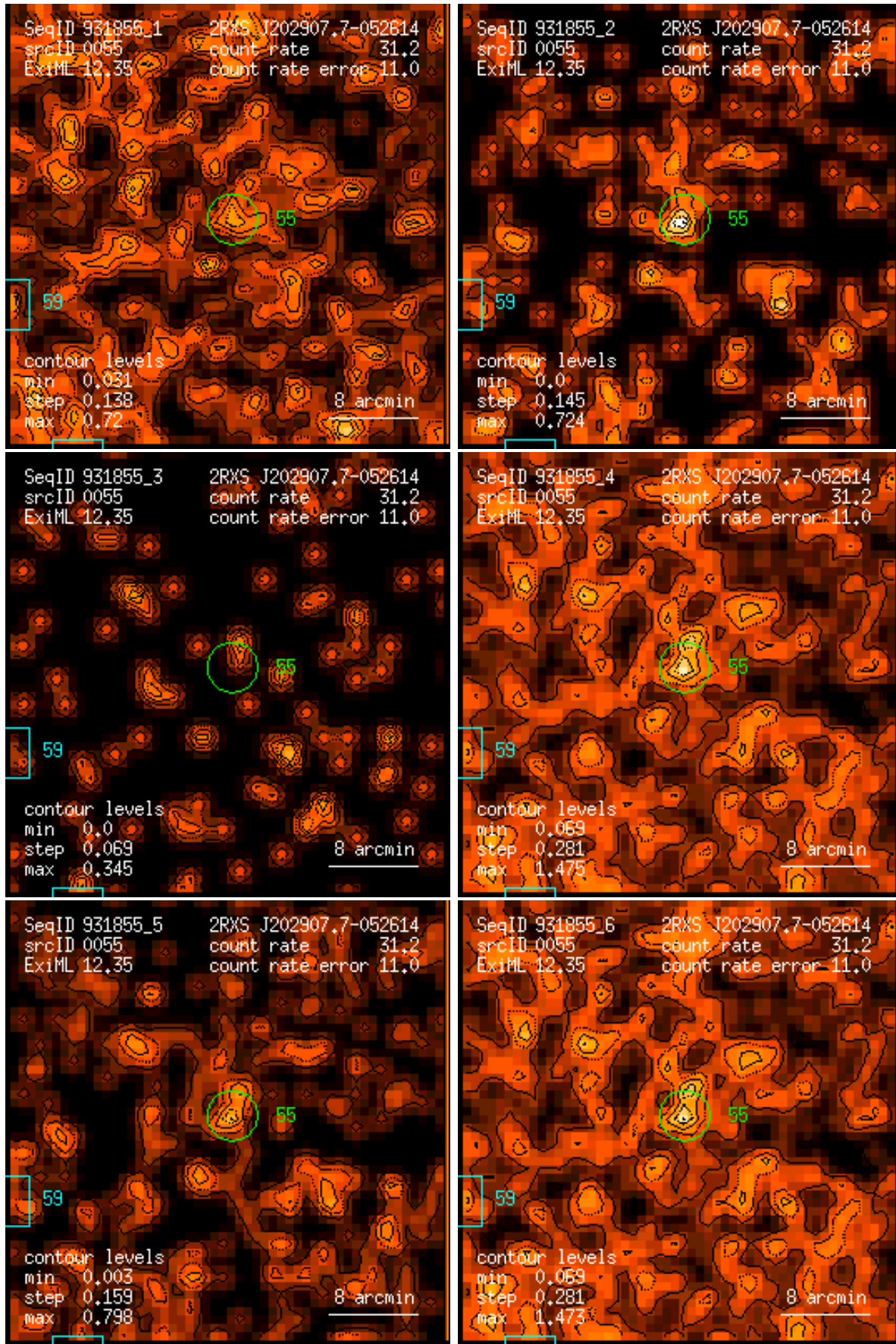
Figure 55: RASS 931855: detection 0055: band rate images, Gaussian filter: (1) PSPC channels 11 – 41, (2) 52 – 90, (3) 91 – 201, (4) 11 – 235, (5) 52 – 201, (6) 11 – 201. Broad band rates in counts/ks. Band rate contour levels in counts/ks/arcmin 2 .
