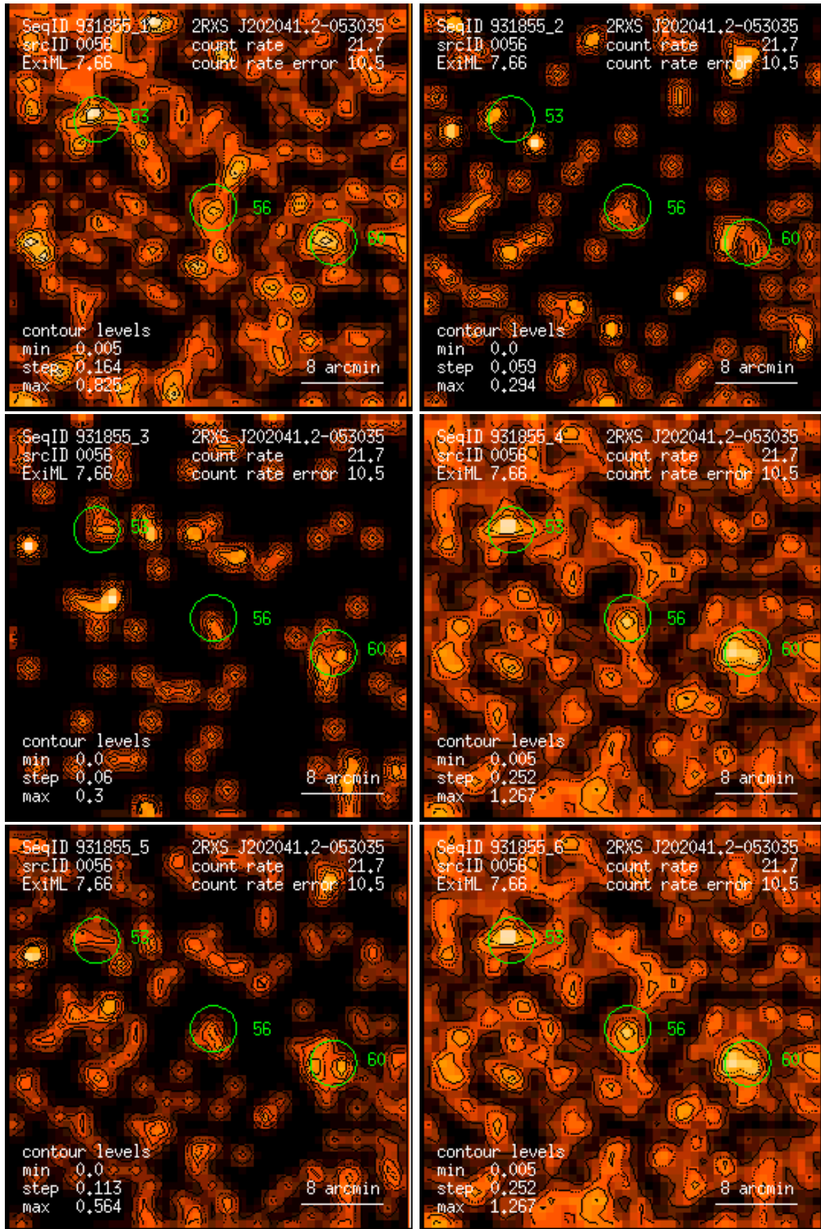
Figure 56: RASS 931855: detection 0056: band rate images, Gaussian filter: (1) PSPC channels 11 – 41, (2) 52 – 90, (3) 91 – 201, (4) 11 – 235, (5) 52 – 201, (6) 11 – 201. Broad band rates in counts/ks. Band rate contour levels in counts/ks/arcmin 2 .
