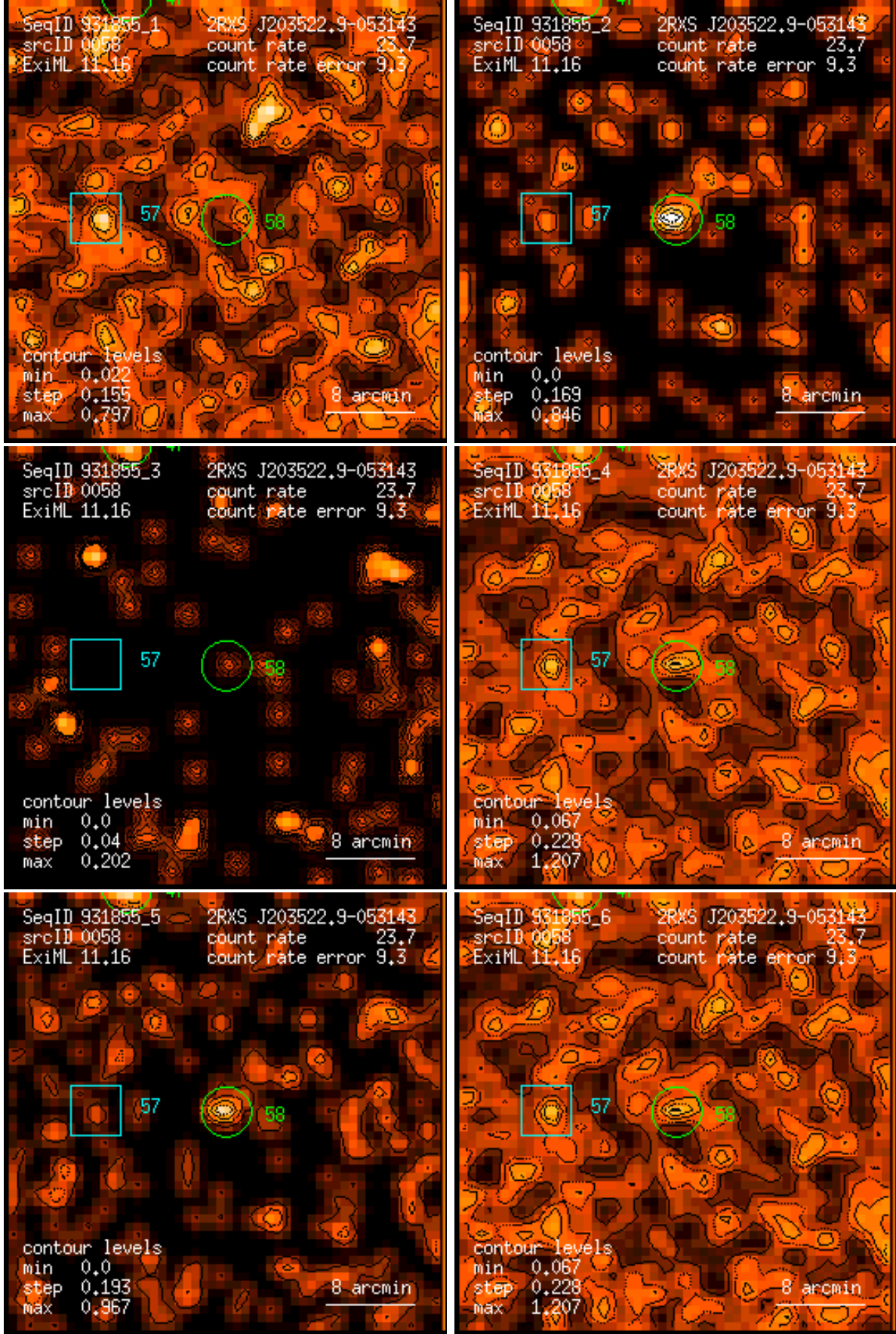
Figure 58: RASS 931855: detection 0058: band rate images, Gaussian filter: (1) PSPC channels 11 – 41, (2) 52 – 90, (3) 91 – 201, (4) 11 – 235, (5) 52 – 201, (6) 11 – 201. Broad band rates in counts/ks. Band rate contour levels in counts/ks/arcmin 2 .
