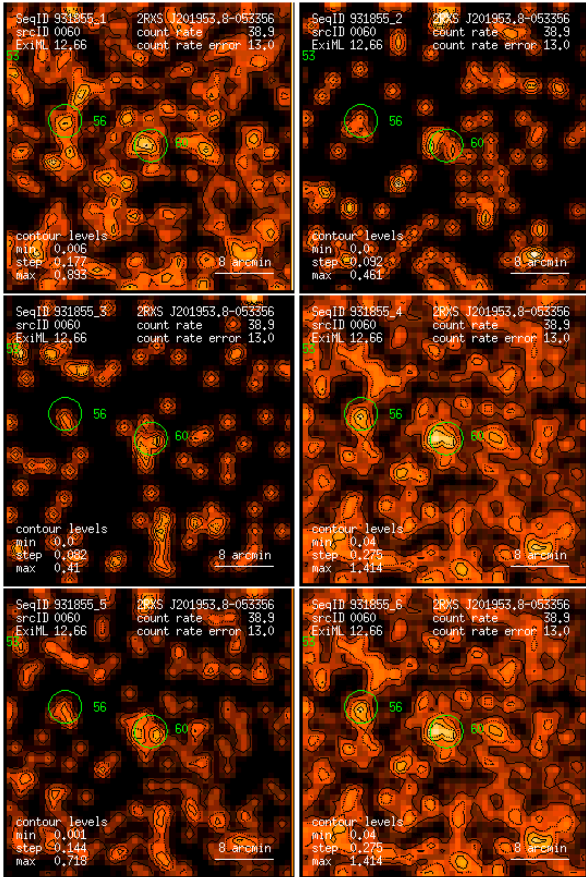
Figure 60: RASS 931855: detection 0060: band rate images, Gaussian filter: (1) PSPC channels 11 – 41, (2) 52 – 90, (3) 91 – 201, (4) 11 – 235, (5) 52 – 201, (6) 11 – 201. Broad band rates in counts/ks. Band rate contour levels in counts/ks/arcmin 2 .
