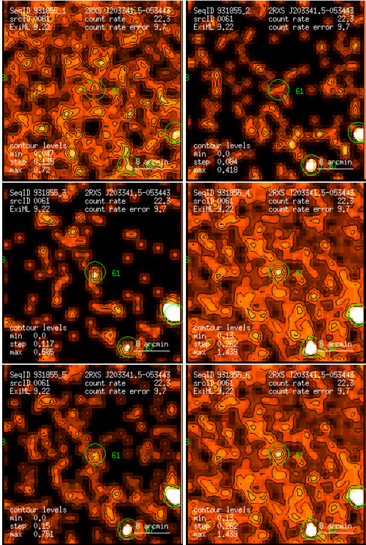
Figure 61: RASS 931855: detection 0061: band rate images, Gaussian filter: (1) PSPC channels 11 – 41, (2) 52 – 90, (3) 91 – 201, (4) 11 – 235, (5) 52 – 201, (6) 11 – 201. Broad band rates in counts/ks. Band rate contour levels in counts/ks/arcmin 2 .
