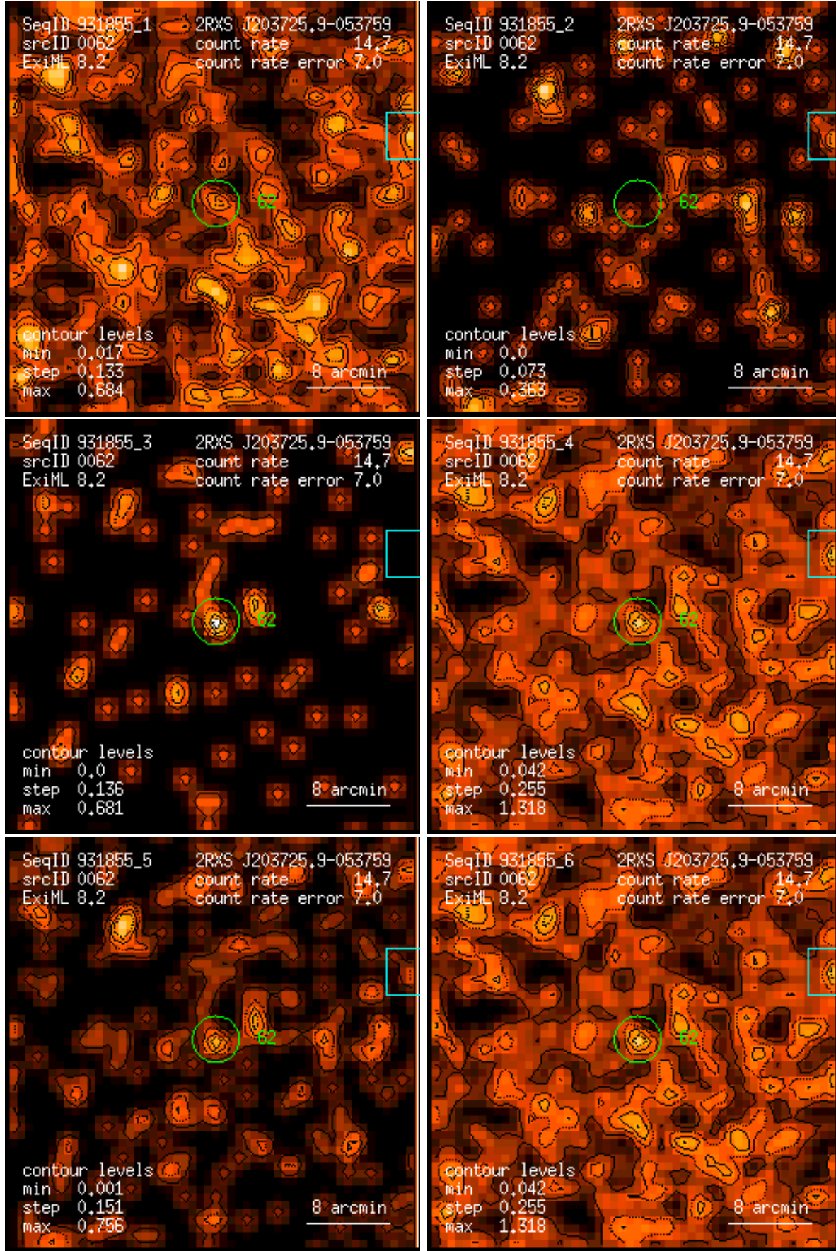
Figure 62: RASS 931855: detection 0062: band rate images, Gaussian filter: (1) PSPC channels 11 – 41, (2) 52 – 90, (3) 91 – 201, (4) 11 – 235, (5) 52 – 201, (6) 11 – 201. Broad band rates in counts/ks. Band rate contour levels in counts/ks/arcmin 2 .
