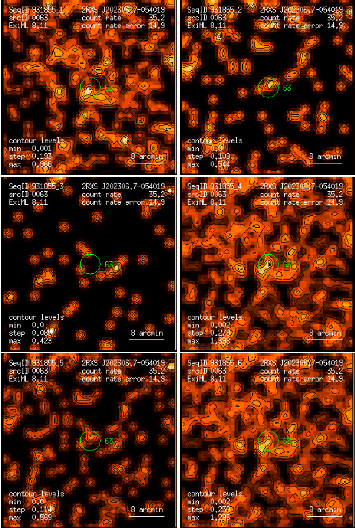
Figure 63: RASS 931855: detection 0063: band rate images, Gaussian filter: (1) PSPC channels 11 – 41, (2) 52 – 90, (3) 91 – 201, (4) 11 – 235, (5) 52 – 201, (6) 11 – 201. Broad band rates in counts/ks. Band rate contour levels in counts/ks/arcmin 2 .
