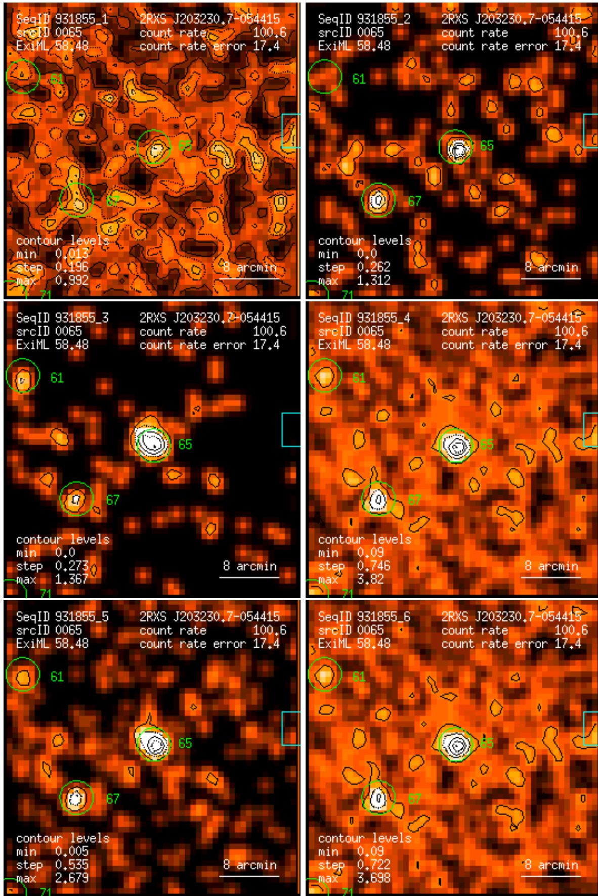
Figure 65: RASS 931855: detection 0065: band rate images, Gaussian filter: (1) PSPC channels 11 – 41, (2) 52 – 90, (3) 91 – 201, (4) 11 – 235, (5) 52 – 201, (6) 11 – 201. Broad band rates in counts/ks. Band rate contour levels in counts/ks/arcmin 2 .
