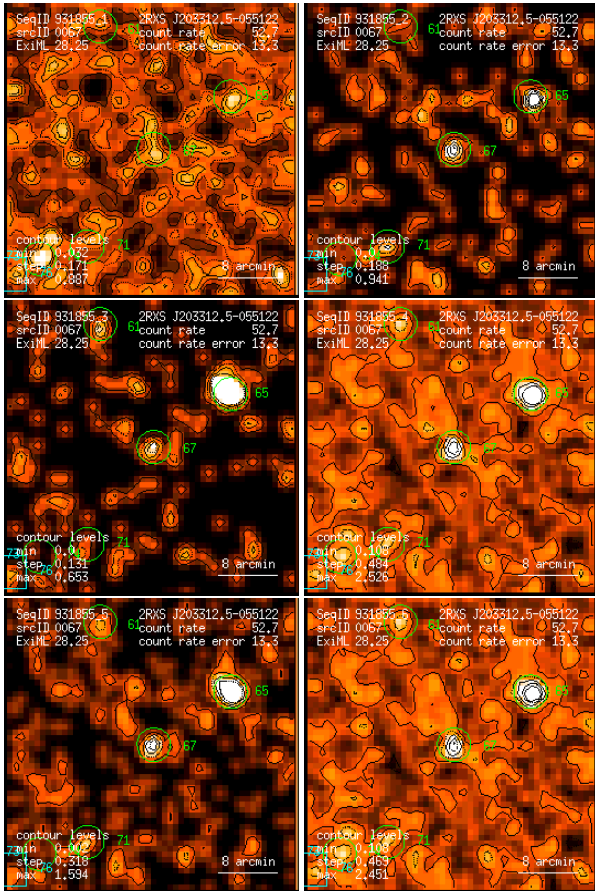
Figure 67: RASS 931855: detection 0067: band rate images, Gaussian filter: (1) PSPC channels 11 – 41, (2) 52 – 90, (3) 91 – 201, (4) 11 – 235, (5) 52 – 201, (6) 11 – 201. Broad band rates in counts/ks. Band rate contour levels in counts/ks/arcmin 2 .
