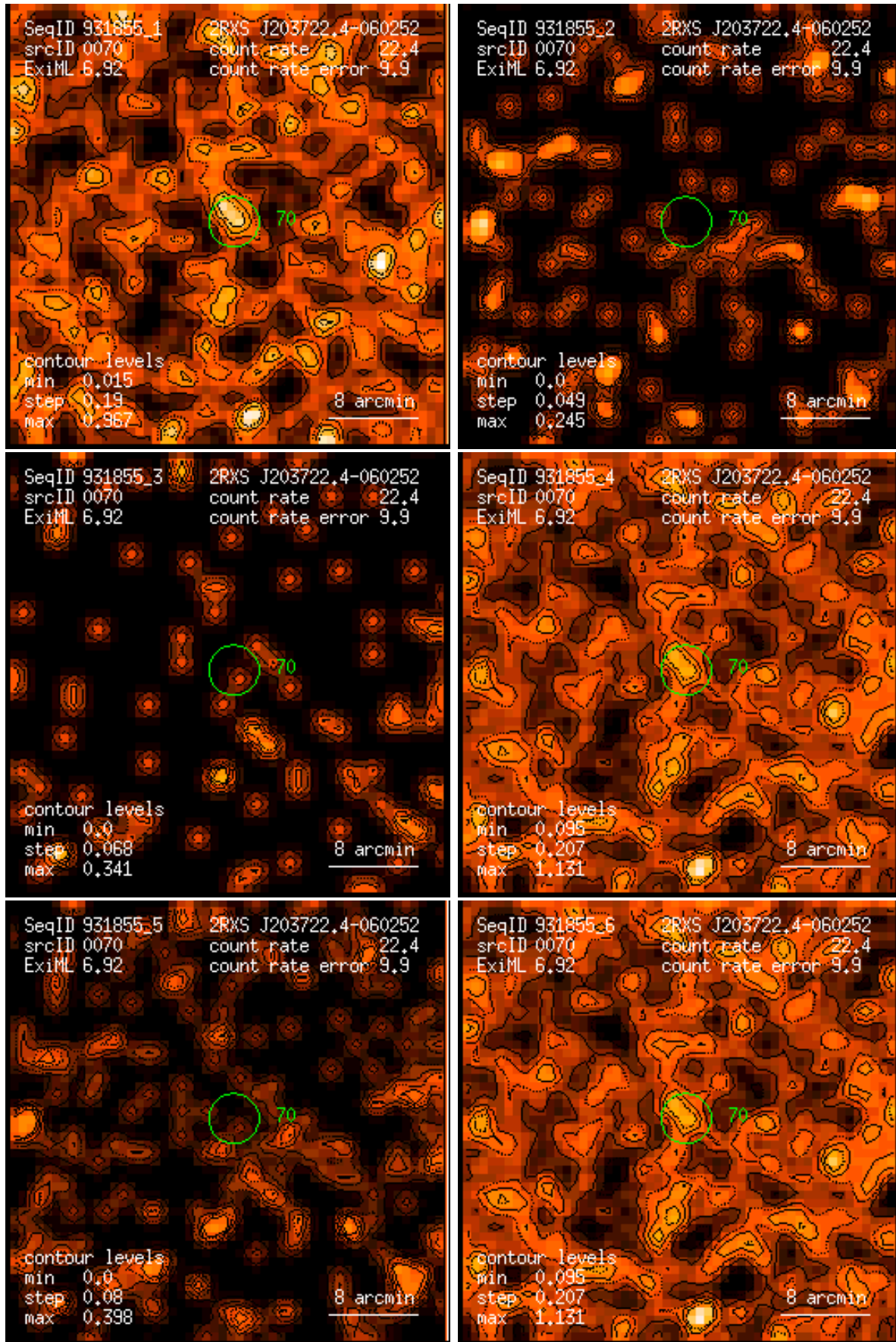
Figure 70: RASS 931855: detection 0070: band rate images, Gaussian filter: (1) PSPC channels 11 – 41, (2) 52 – 90, (3) 91 – 201, (4) 11 – 235, (5) 52 – 201, (6) 11 – 201. Broad band rates in counts/ks. Band rate contour levels in counts/ks/arcmin 2 .
