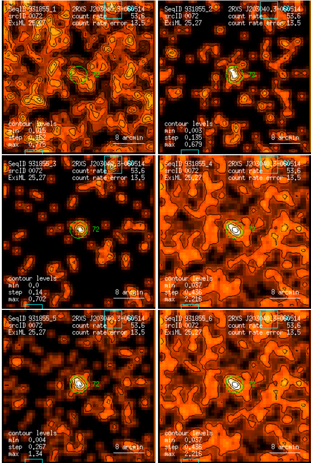
Figure 72: RASS 931855: detection 0072: band rate images, Gaussian filter: (1) PSPC channels 11 – 41, (2) 52 – 90, (3) 91 – 201, (4) 11 – 235, (5) 52 – 201, (6) 11 – 201. Broad band rates in counts/ks. Band rate contour levels in counts/ks/arcmin 2 .
