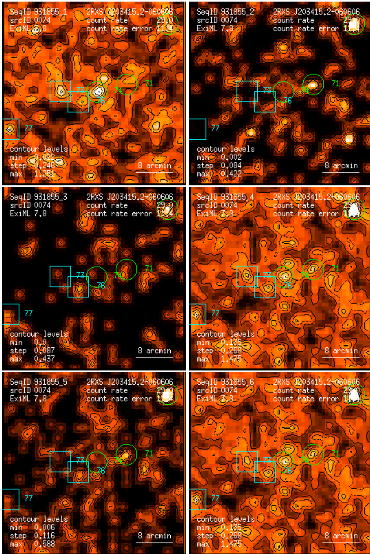
Figure 74: RASS 931855: detection 0074: band rate images, Gaussian filter: (1) PSPC channels 11 – 41, (2) 52 – 90, (3) 91 – 201, (4) 11 – 235, (5) 52 – 201, (6) 11 – 201. Broad band rates in counts/ks. Band rate contour levels in counts/ks/arcmin 2 .
