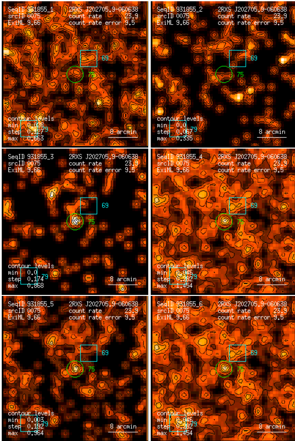
Figure 75: RASS 931855: detection 0075: band rate images, Gaussian filter: (1) PSPC channels 11 – 41, (2) 52 – 90, (3) 91 – 201, (4) 11 – 235, (5) 52 – 201, (6) 11 – 201. Broad band rates in counts/ks. Band rate contour levels in counts/ks/arcmin 2 .
