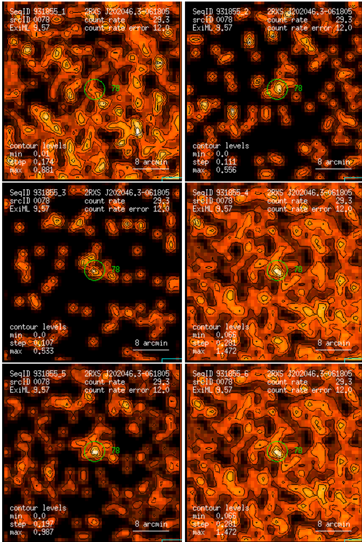
Figure 78: RASS 931855: detection 0078: band rate images, Gaussian filter: (1) PSPC channels 11 – 41, (2) 52 – 90, (3) 91 – 201, (4) 11 – 235, (5) 52 – 201, (6) 11 – 201. Broad band rates in counts/ks. Band rate contour levels in counts/ks/arcmin 2 .
