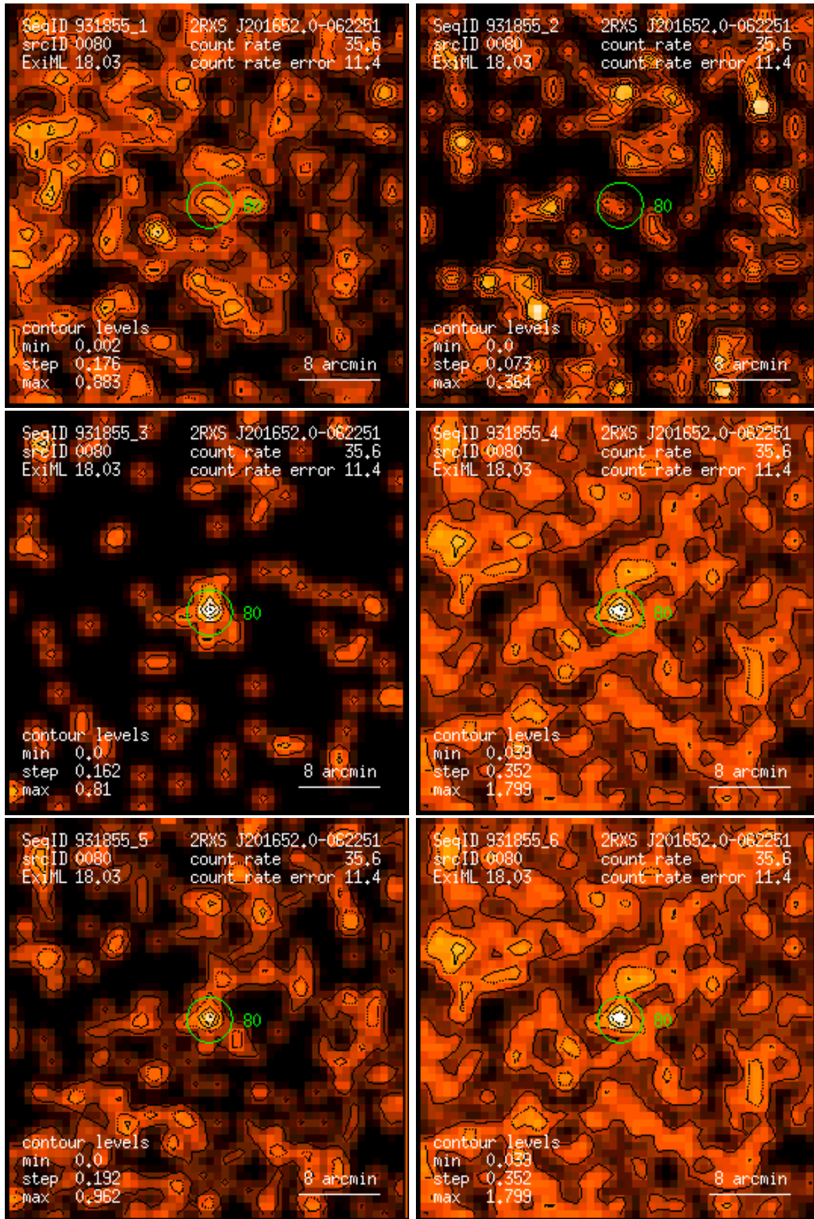
Figure 80: RASS 931855: detection 0080: band rate images, Gaussian filter: (1) PSPC channels 11 – 41, (2) 52 – 90, (3) 91 – 201, (4) 11 – 235, (5) 52 – 201, (6) 11 – 201. Broad band rates in counts/ks. Band rate contour levels in counts/ks/arcmin 2 .
