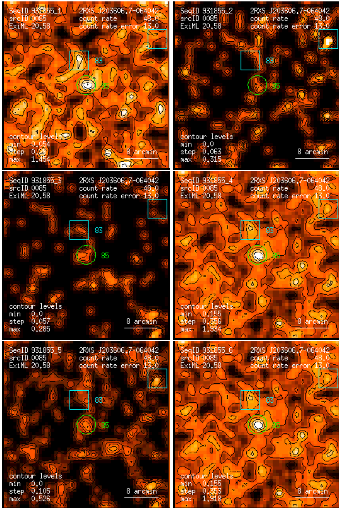
Figure 85: RASS 931855: detection 0085: band rate images, Gaussian filter: (1) PSPC channels 11 – 41, (2) 52 – 90, (3) 91 – 201, (4) 11 – 235, (5) 52 – 201, (6) 11 – 201. Broad band rates in counts/ks. Band rate contour levels in counts/ks/arcmin 2 .
