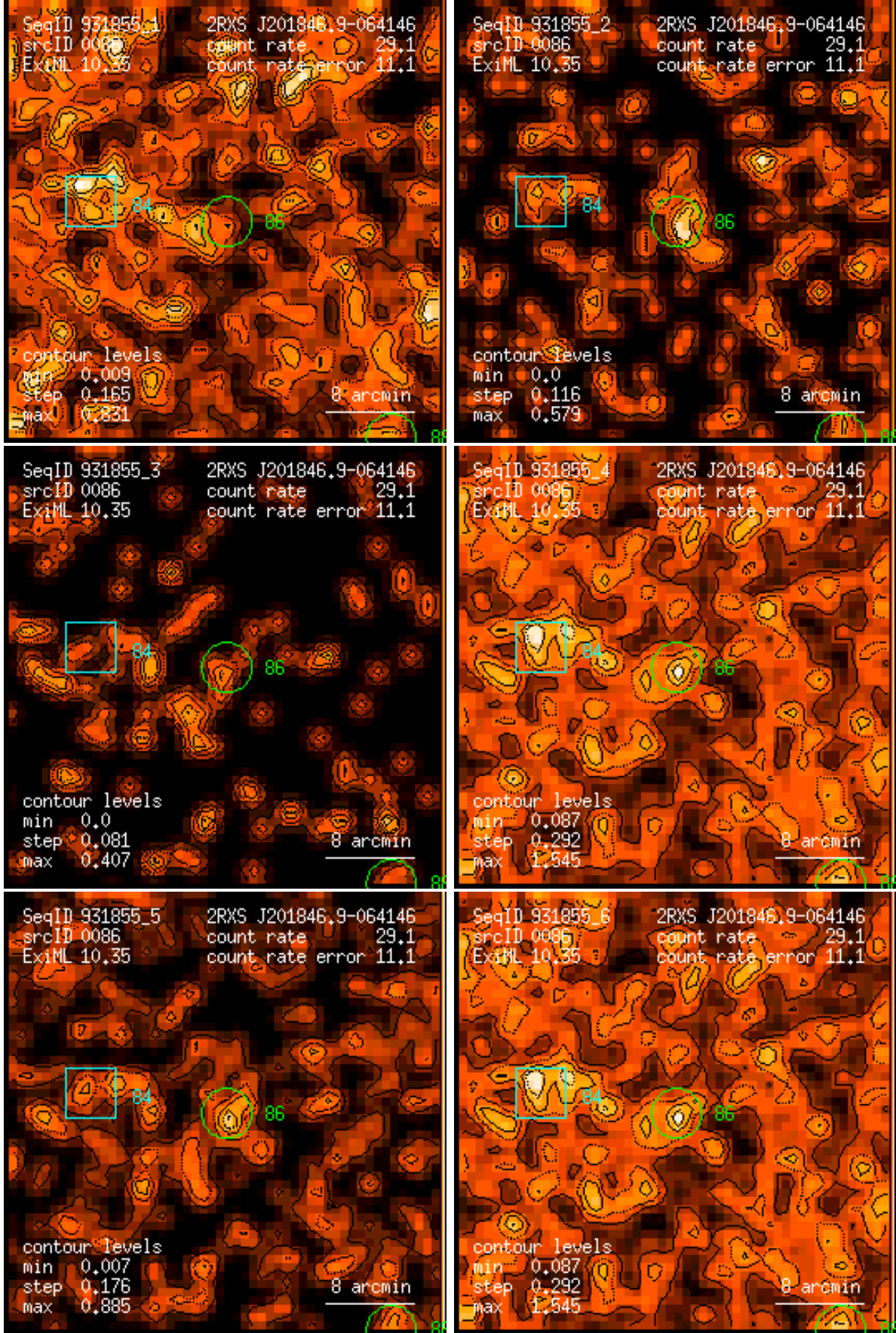
Figure 86: RASS 931855: detection 0086: band rate images, Gaussian filter: (1) PSPC channels 11 – 41, (2) 52 – 90, (3) 91 – 201, (4) 11 – 235, (5) 52 – 201, (6) 11 – 201. Broad band rates in counts/ks. Band rate contour levels in counts/ks/arcmin 2 .
