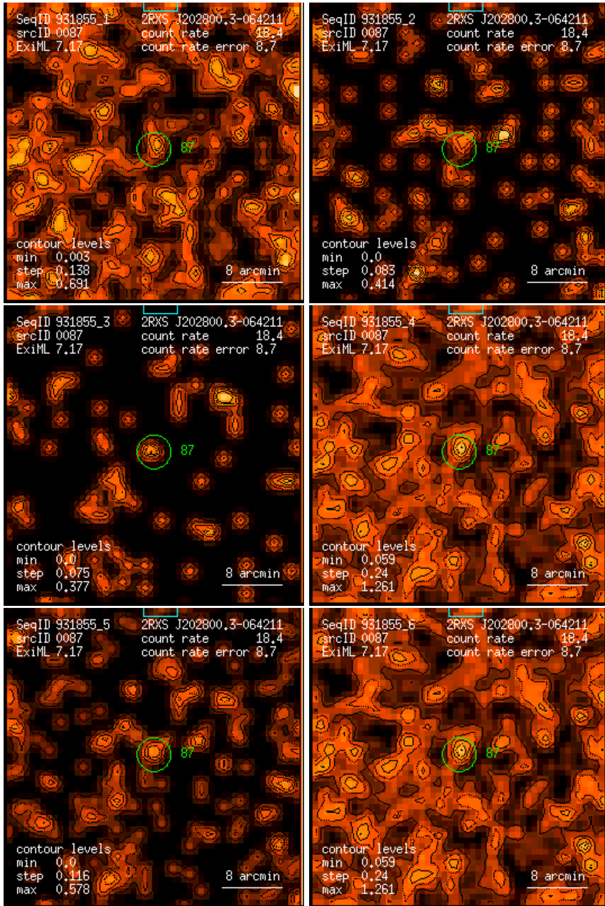
Figure 87: RASS 931855: detection 0087: band rate images, Gaussian filter: (1) PSPC channels 11 – 41, (2) 52 – 90, (3) 91 – 201, (4) 11 – 235, (5) 52 – 201, (6) 11 – 201. Broad band rates in counts/ks. Band rate contour levels in counts/ks/arcmin 2 .
